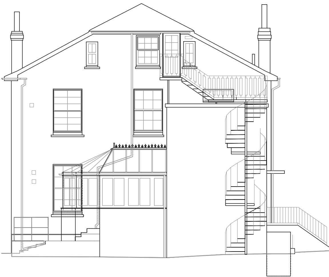
South East Elevation (Rear) 1:100
