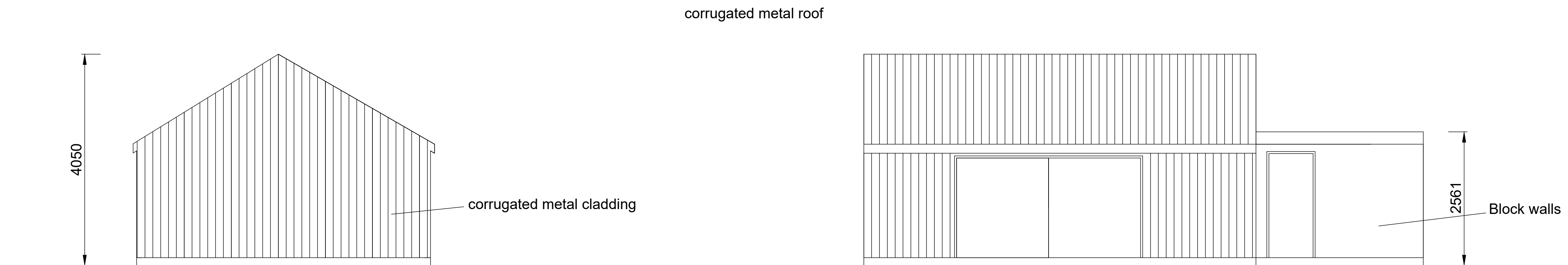
Side Elevation (East)
