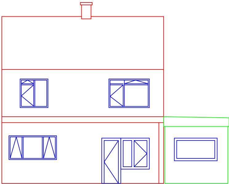
PROPOSED REAR ELEVATON - NORTH
