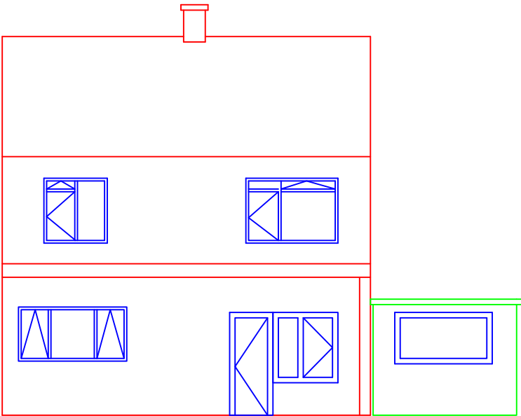
EXISTING REAR ELEVATON - NORTH
