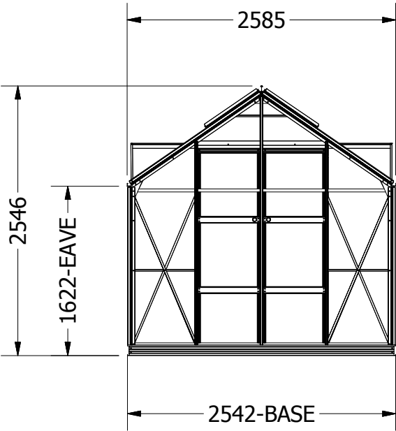
REAR VIEW
