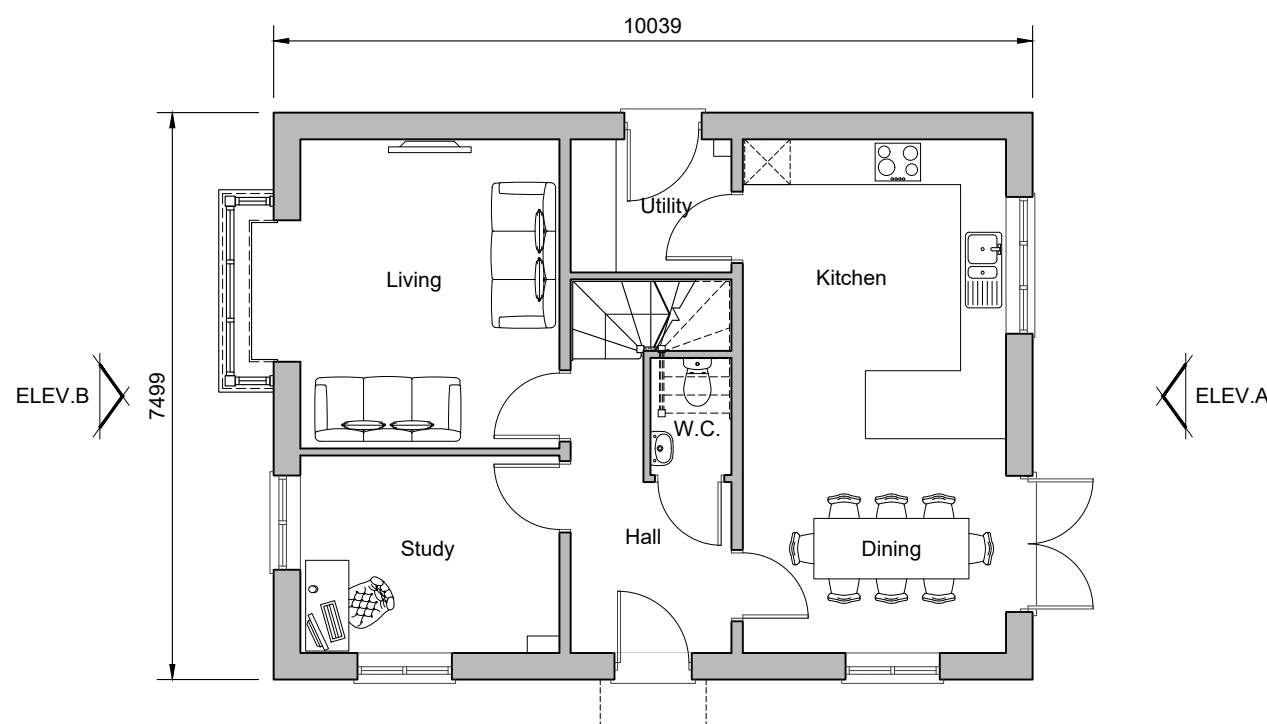
Ground Floor Plan Plot 66 Plot 20 (handed)
