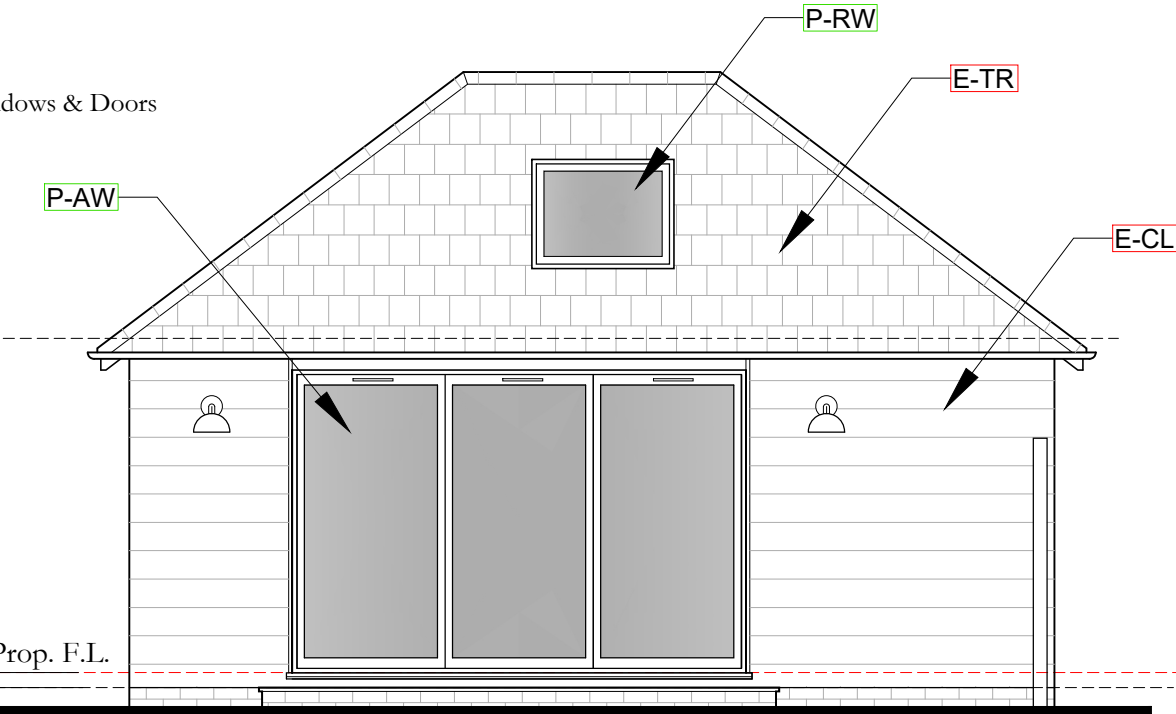
PROPOSED ELEVATION- SIDE SCALE 1 : 50 @ A3
