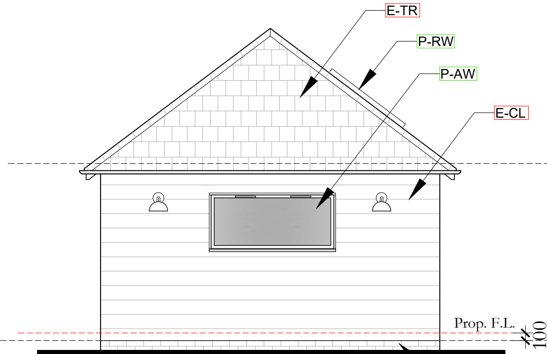
PROPOSED ELEVATION- REAR SCALE 1 : 50 @ A3
