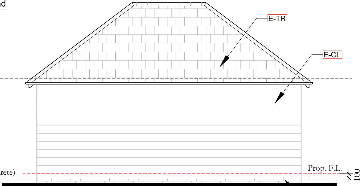
PROPOSED ELEVATION- SIDE SCALE 1 : 50 @ A3
