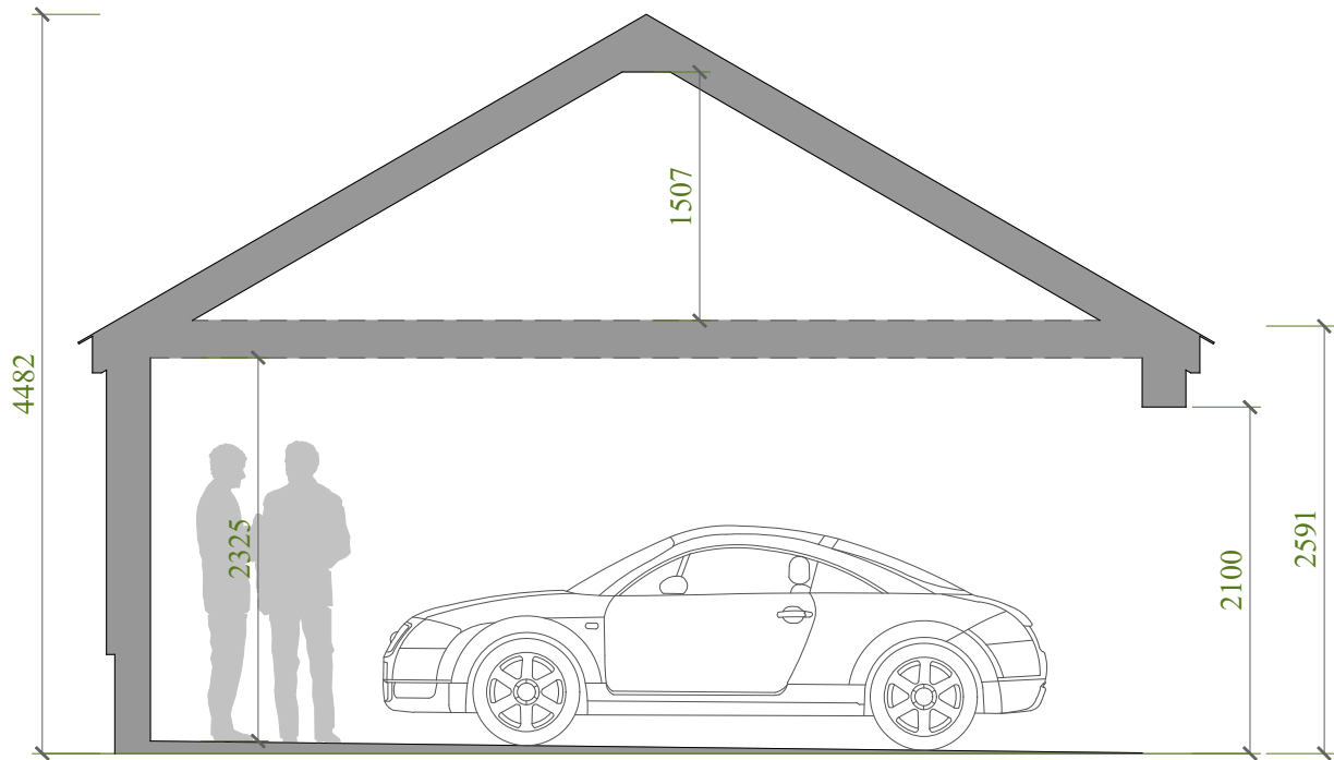
Garage Section BB
