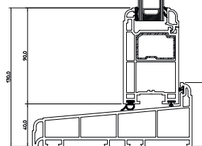
Sideways View - Deep Bottom Rail
