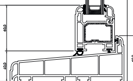
Sideways View - Standard Bottom Rail
