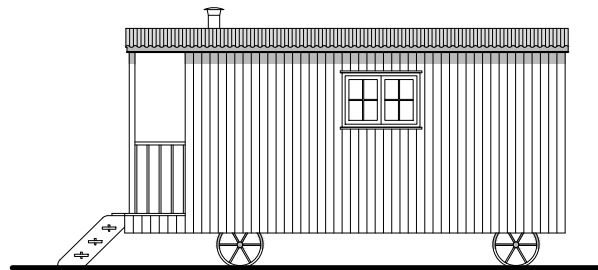
North elevation
