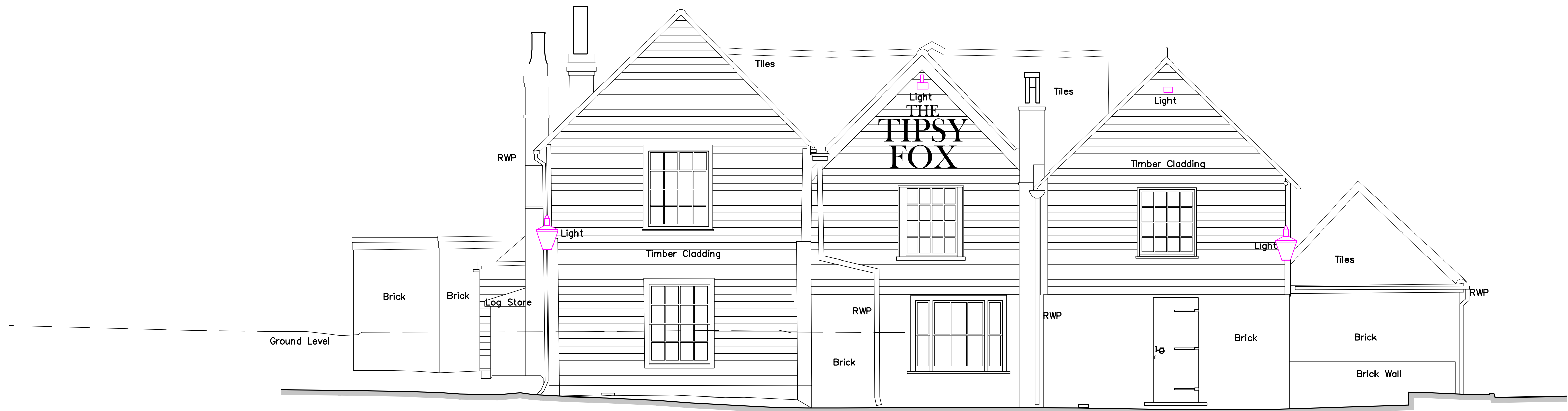
EXISTING EAST ELEVATION
