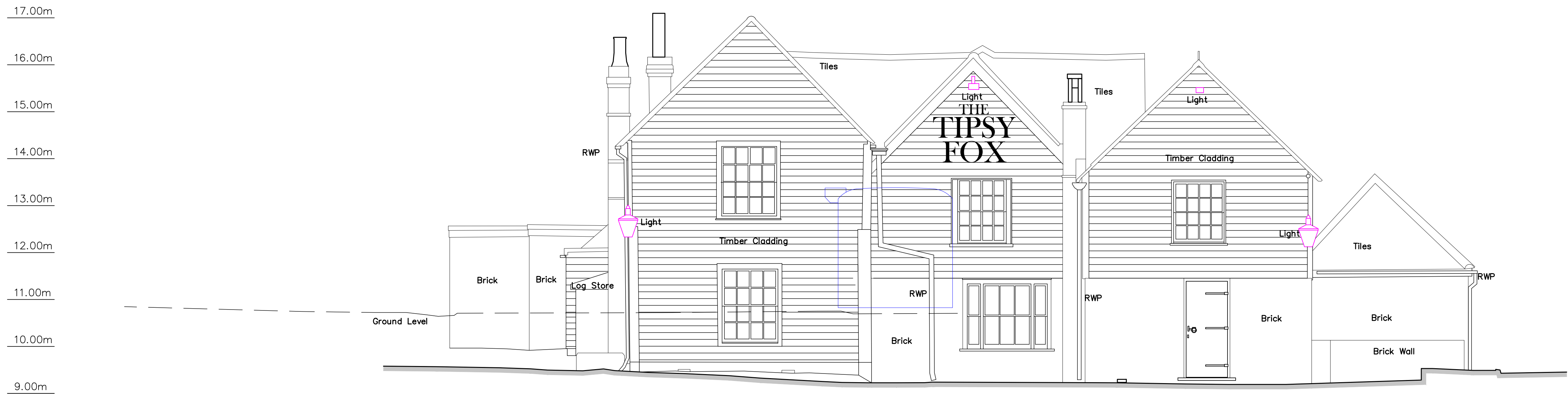
EXISTING AS BUILT EAST ELEVATION
