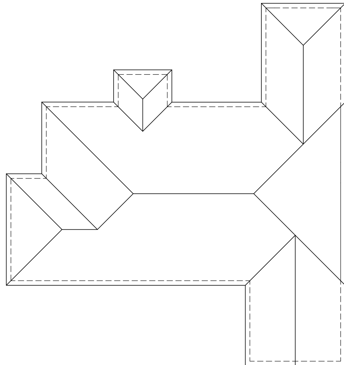
Proposed Roof layout
