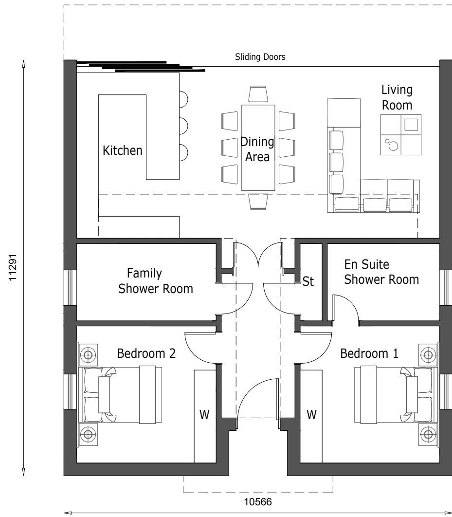
Ground Floor GEA - 117.3 m2
