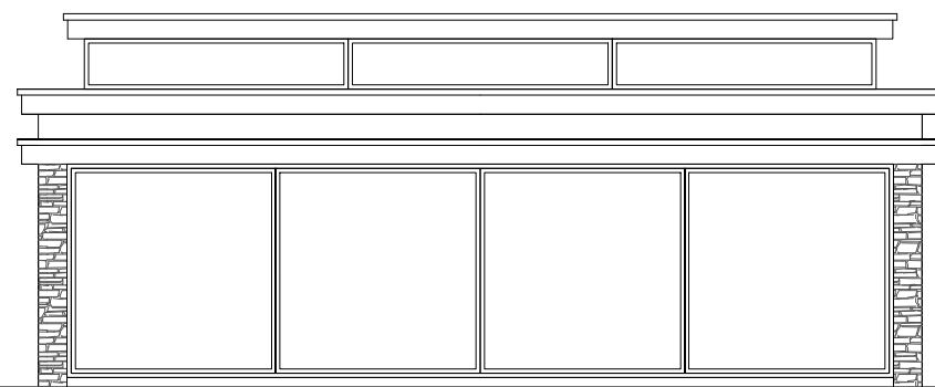
Rear Elevation
