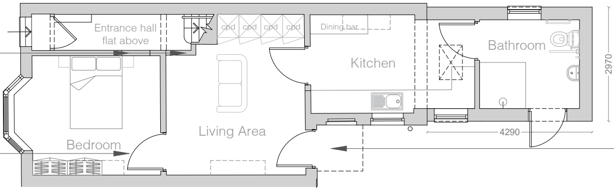
Proposed Ground Floor Plan (Flat 1)
