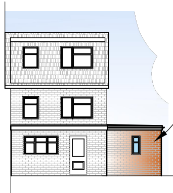
03 Rear Elevation - As Proposed 3000 1:200 (at A3)
