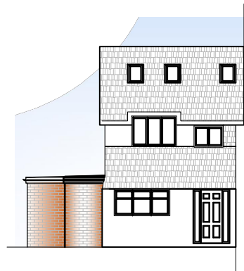
01 Front Elevation - As Proposed 3000 1:200 (at A3)
