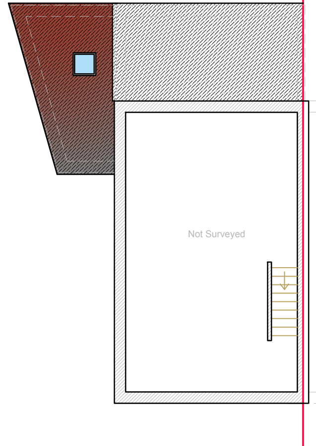
06 First floor plan - As Proposed 3000 1:100 (at A3)
