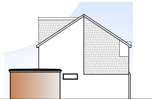
02 Side Elevation - As Proposed 3000 1:200 (at A3)
