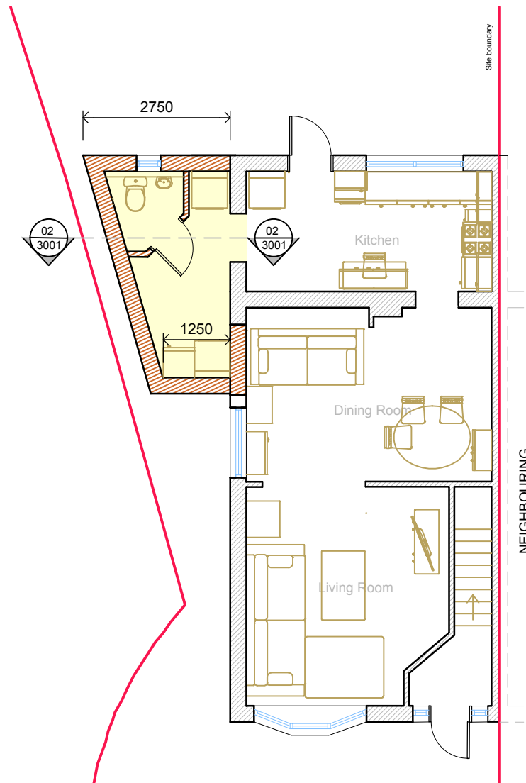
05 Ground floor plan - As Proposed 3000 1:100 (at A3)
