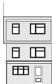
02 Side Elevation - As Existing 2000 1:200 (at A3)
