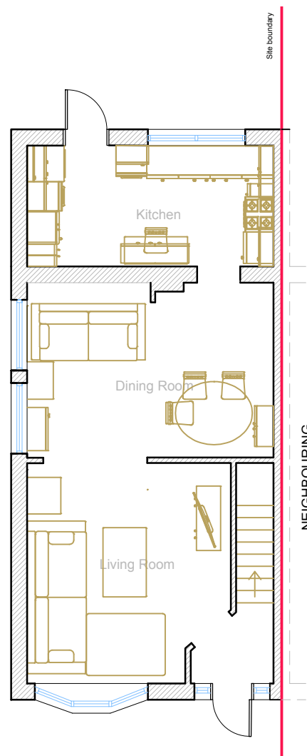
05 Ground floor plan - As Existing 2000 1:100 (at A3)
