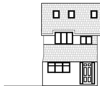
01 Front Elevation - As Existing 2000 1:200 (at A3)
