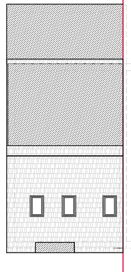
07 Roof plan - As Existing 2000 1:100 (at A3)
