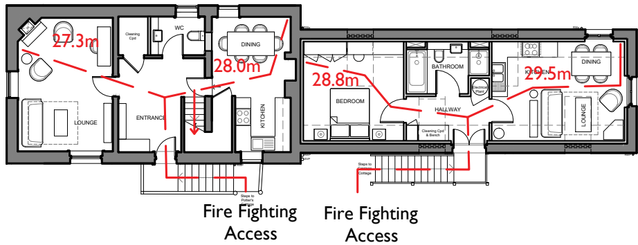
3 Proposed First Floor Fire Fighting Distance Plan to Cottages 6001 Scale - 1:200 @ A3
