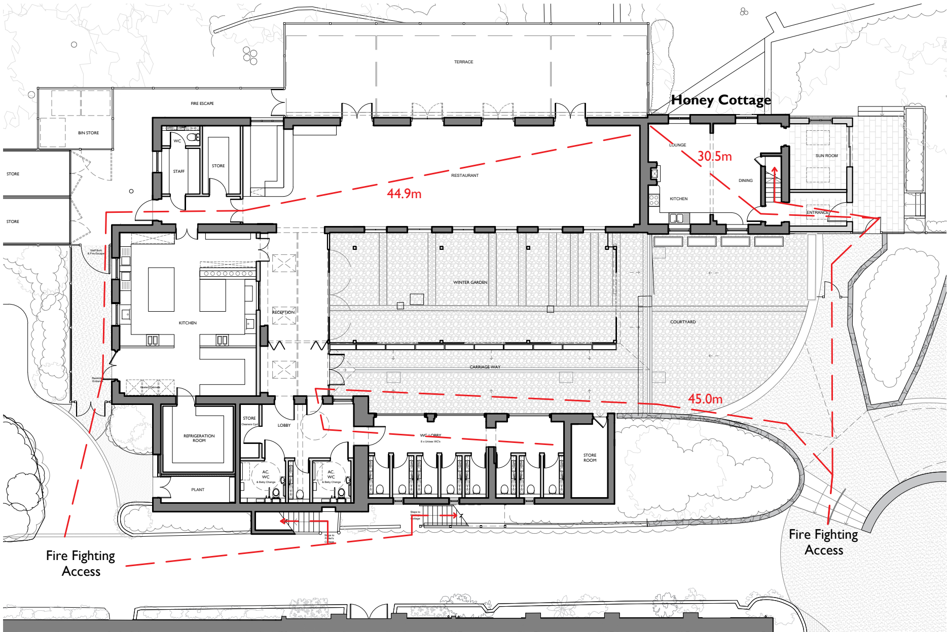
1 Proposed Ground Floor Fire Fighting Distance Plan 6001 Scale - 1:200 @ A3
