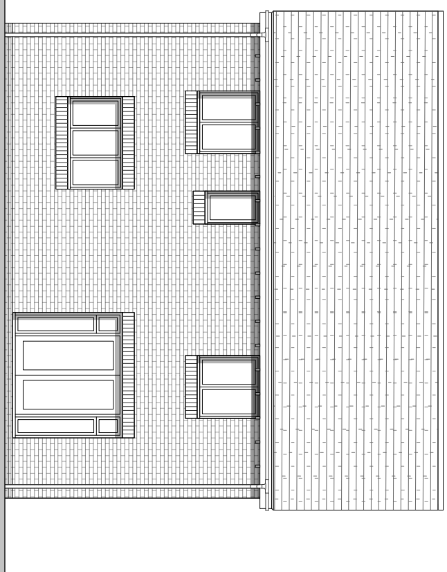
Rear Elevation
