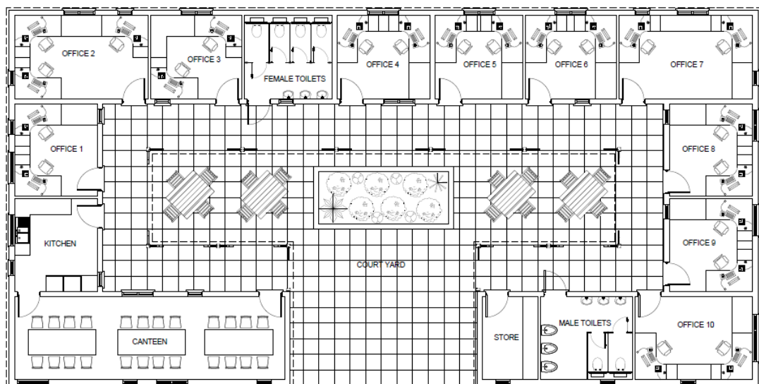
Figure 3.1 Proposed Floor Plan
