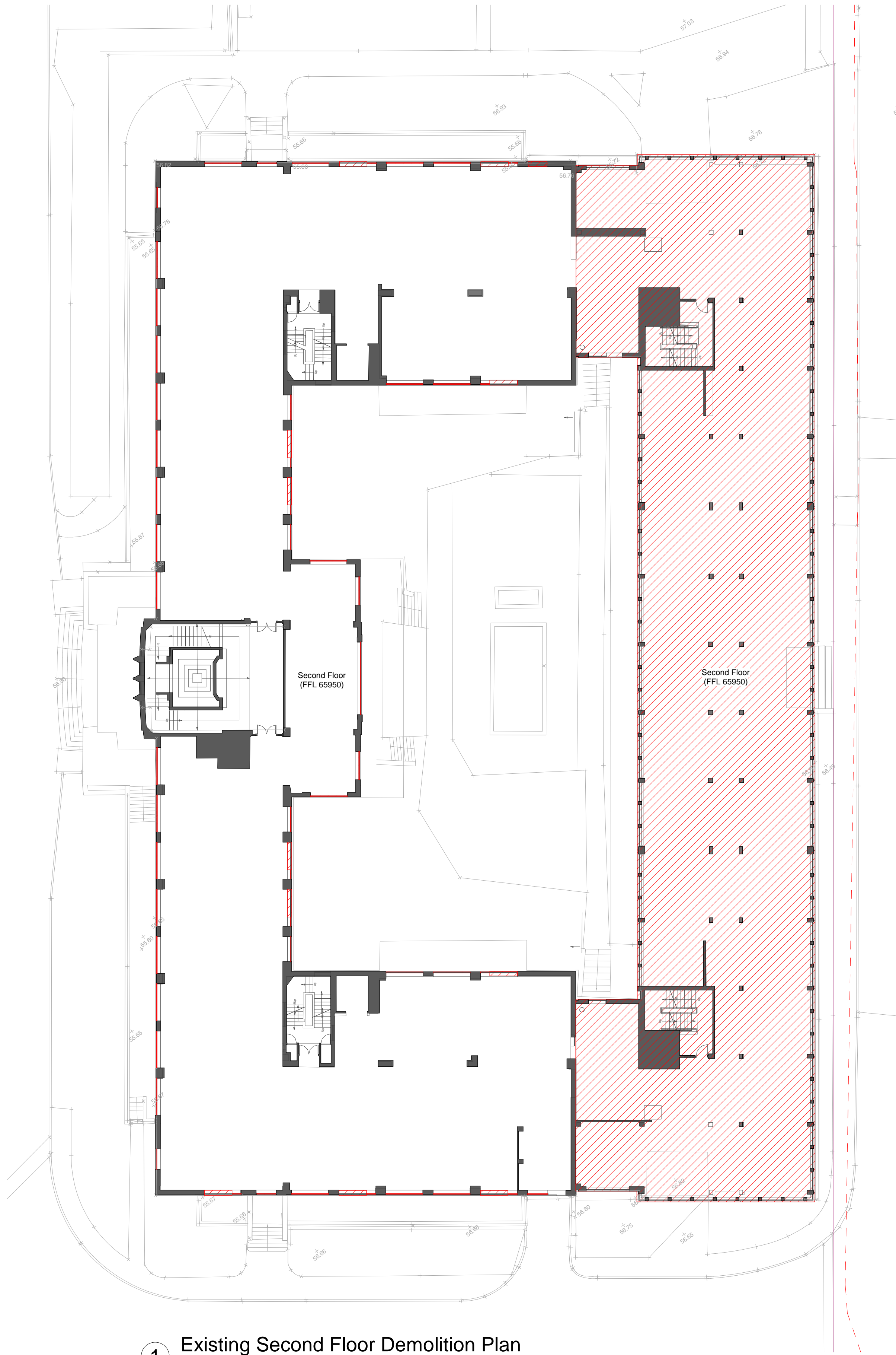
1 Existing Second Floor Demolition Plan 1 : 200
