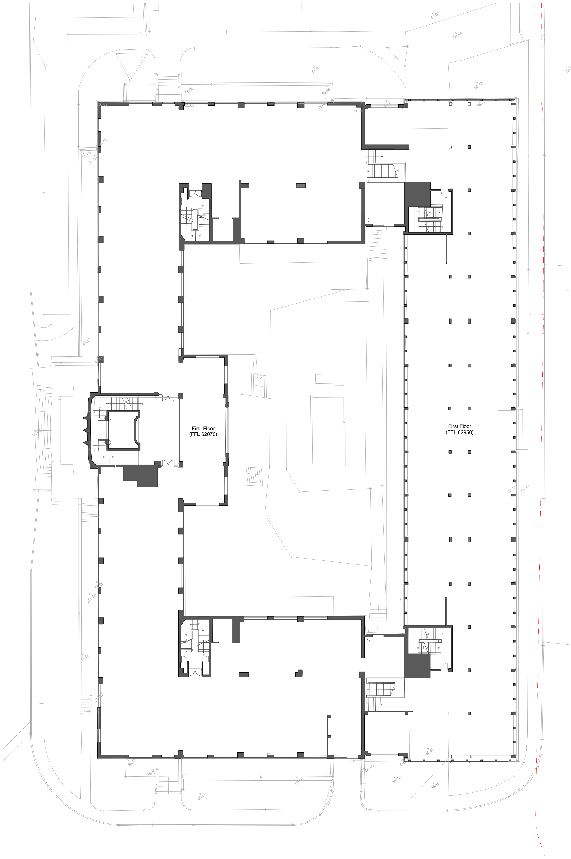
1 Existing First Floor Plan 1 : 200
