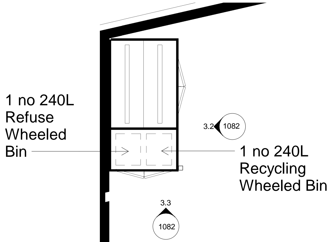
3 Type 3_Plan 1 : 50
