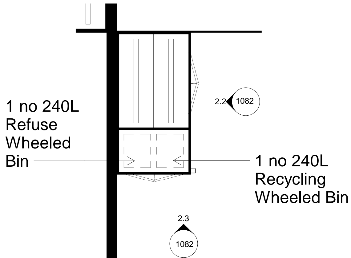
2 Type 2_Plan 1 : 50
