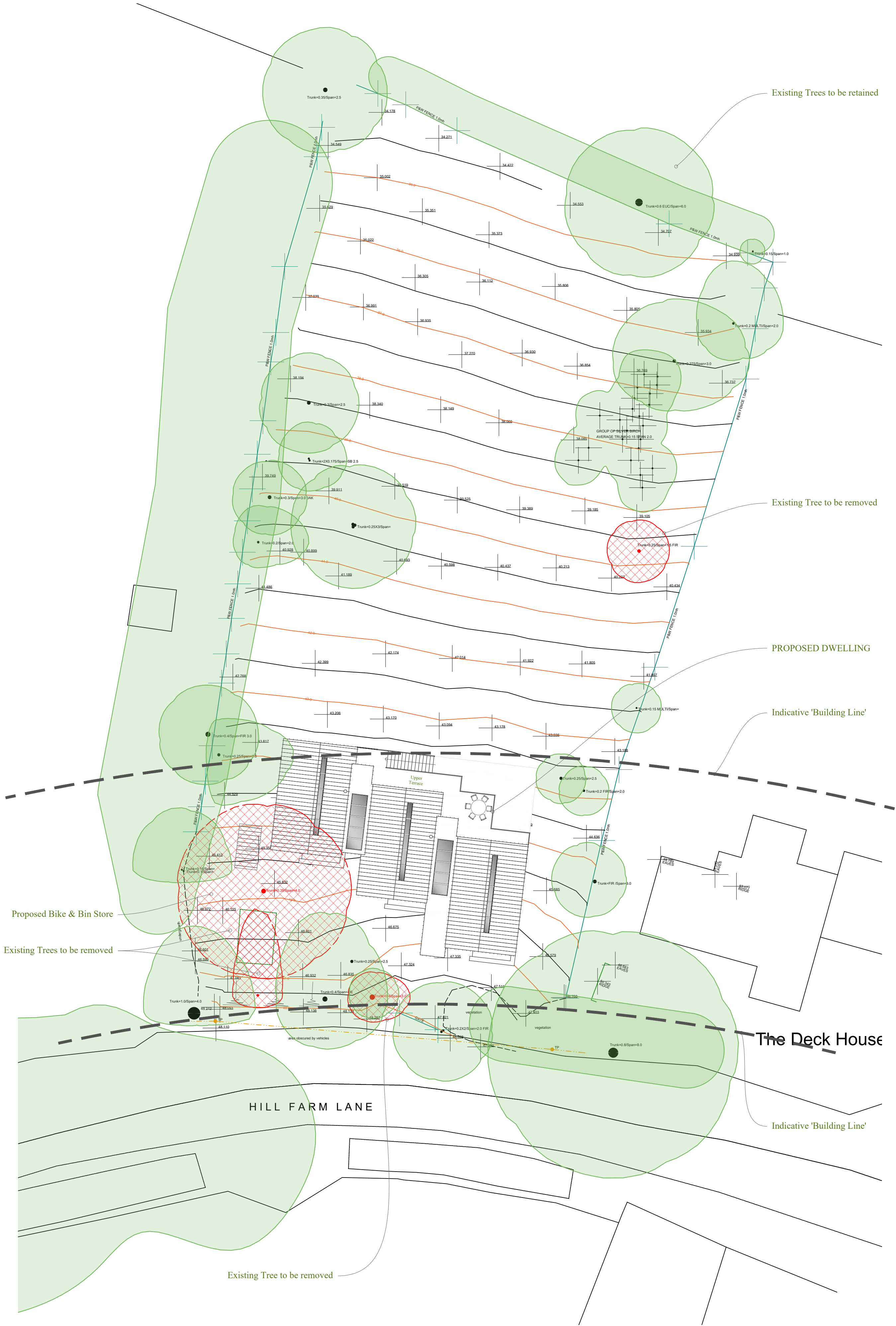
Block Plan 1:200 | PROPOSED
