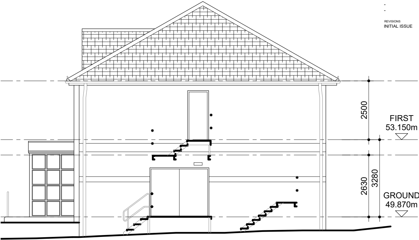
WEST ELEVATION - AS EXISTING AND AS PROPOSED
