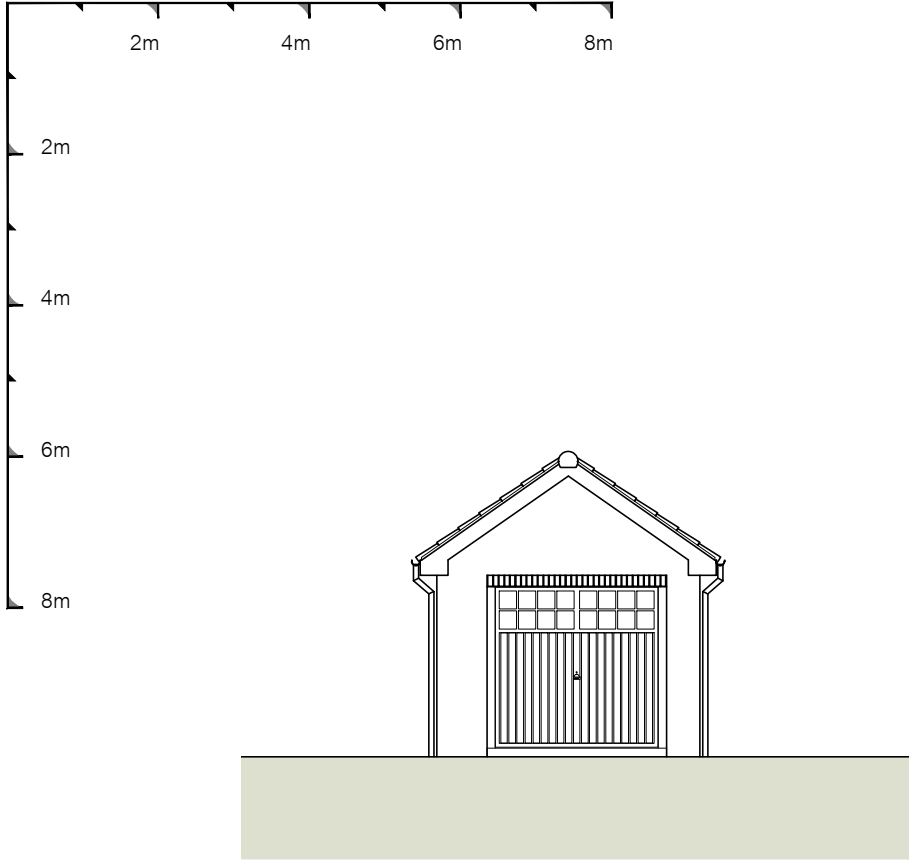
1 Front Elevation 1 : 100
