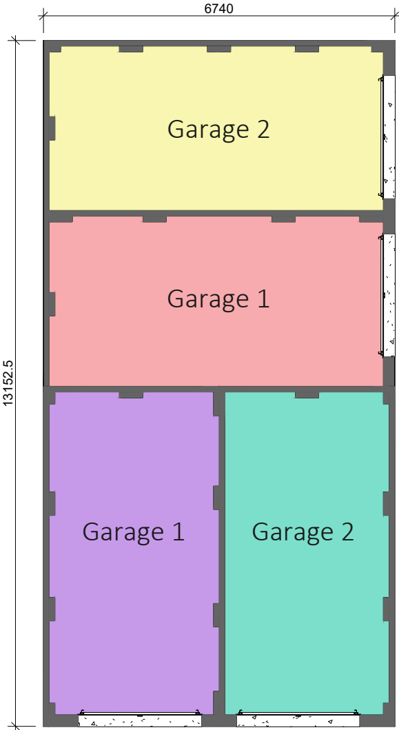
5 Ground Floor 1 : 100
