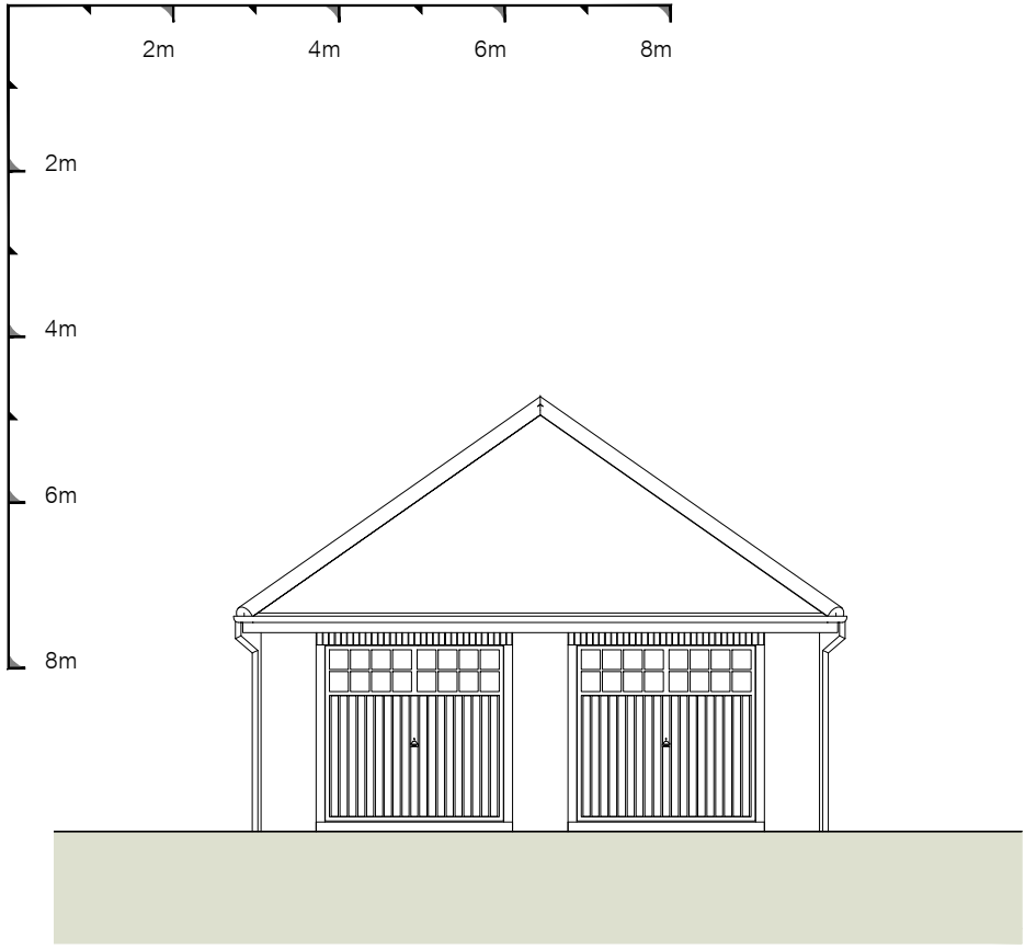
1 Front Elevation 1 : 100
