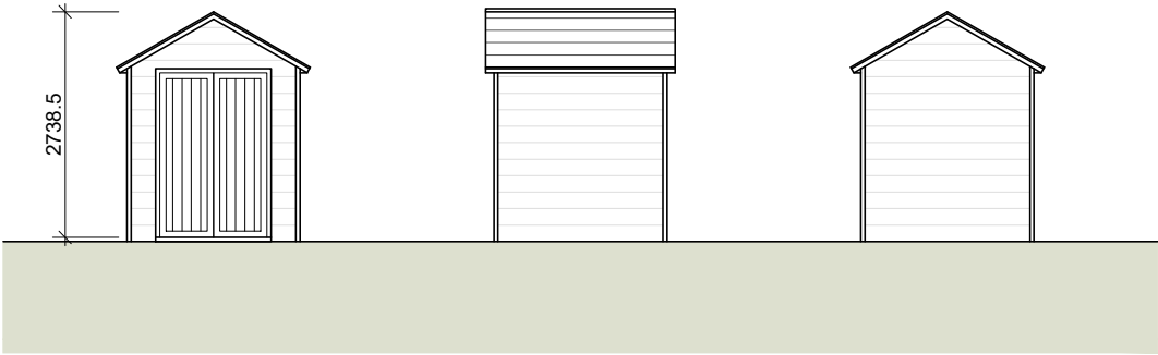
1 Elevations - Double cycle shed 1 : 100
