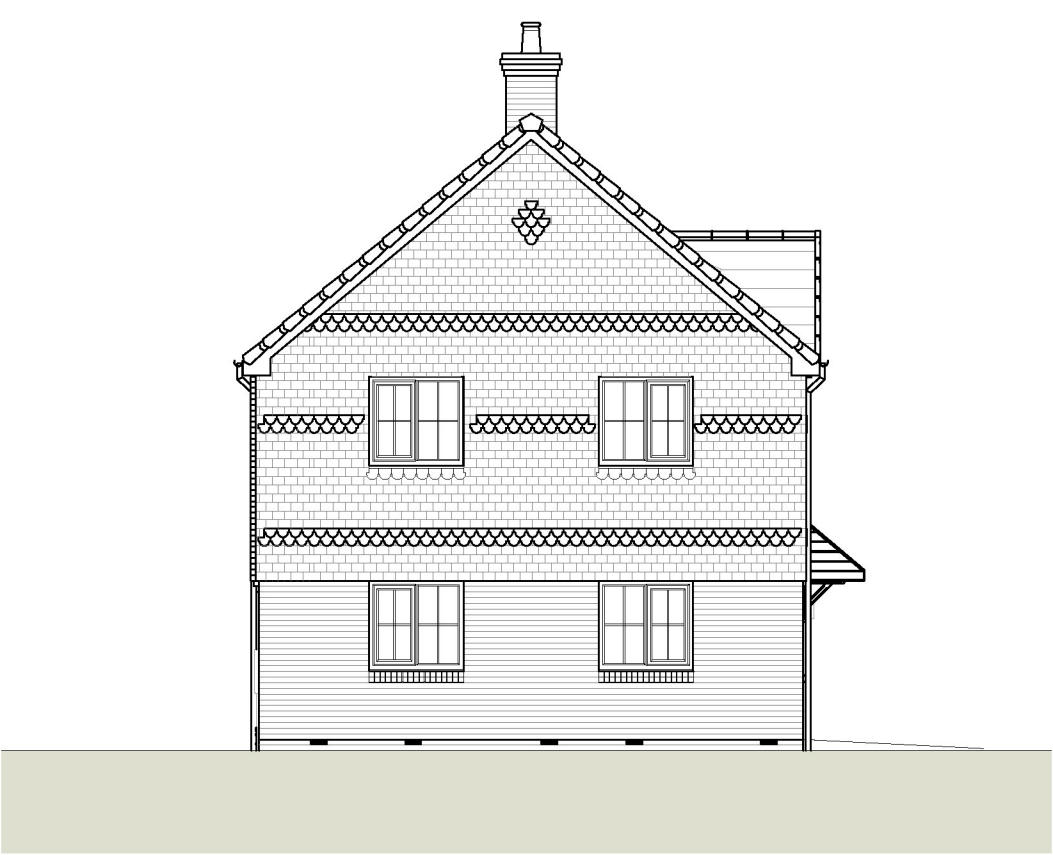
2 Gable Elevation 1 : 100
