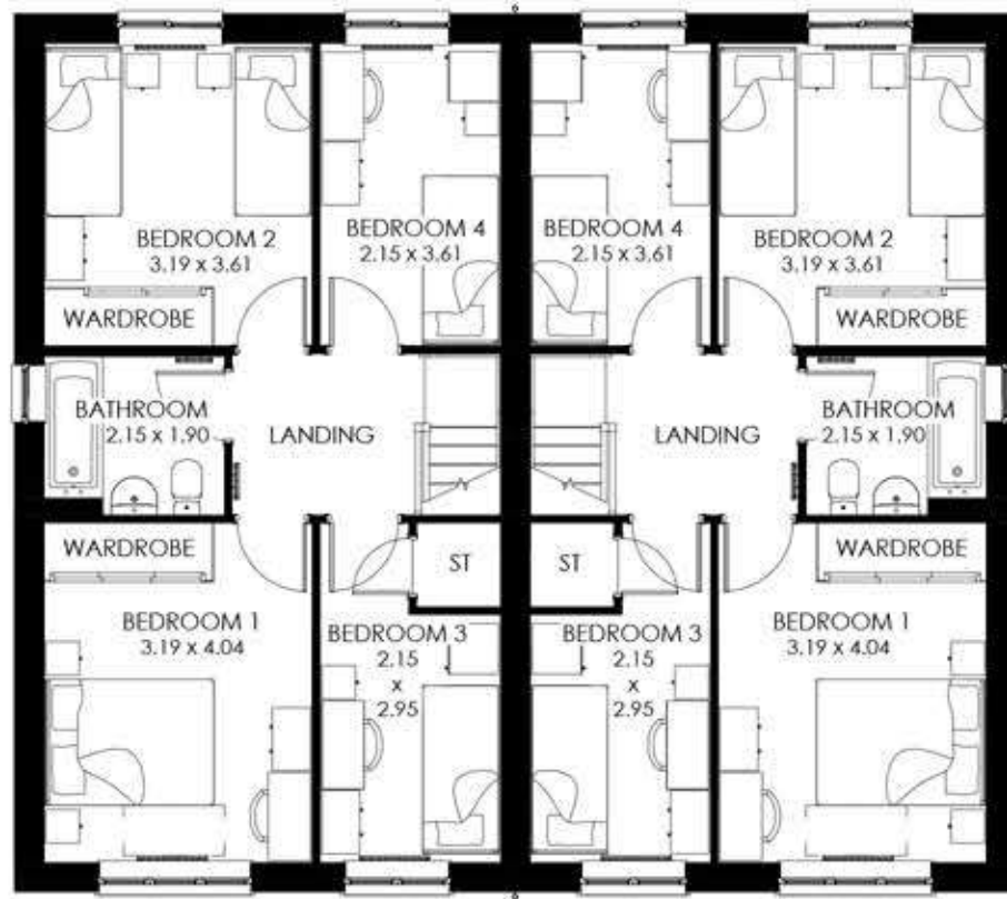
First Floor
