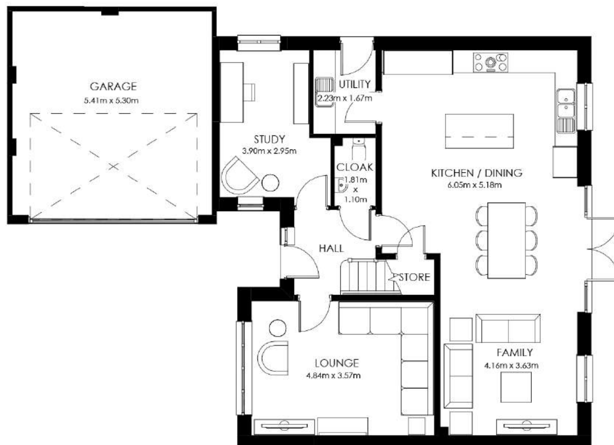
Ground Floor
