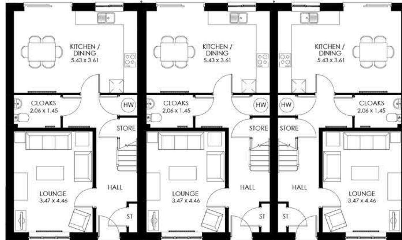
Ground Floor
