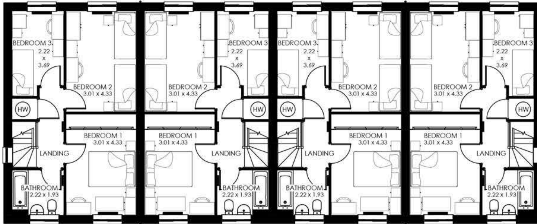
First Floor
