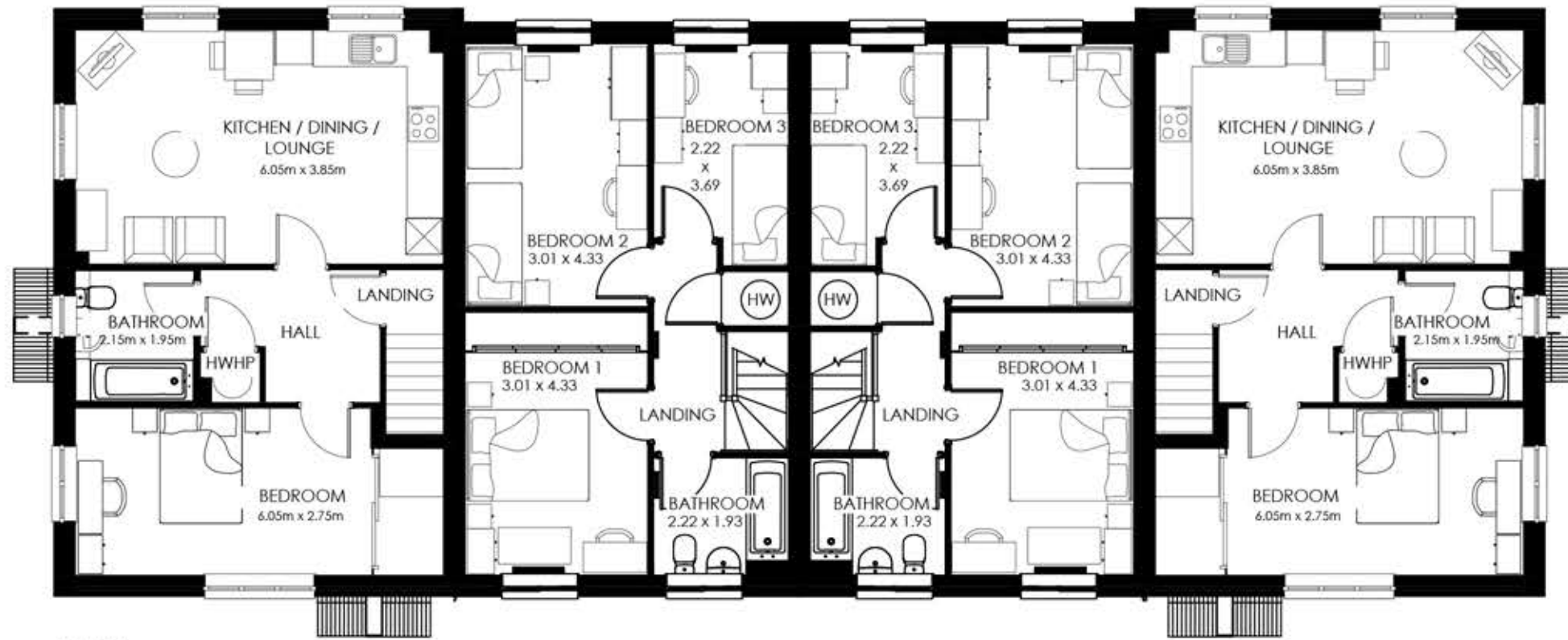
First Floor
