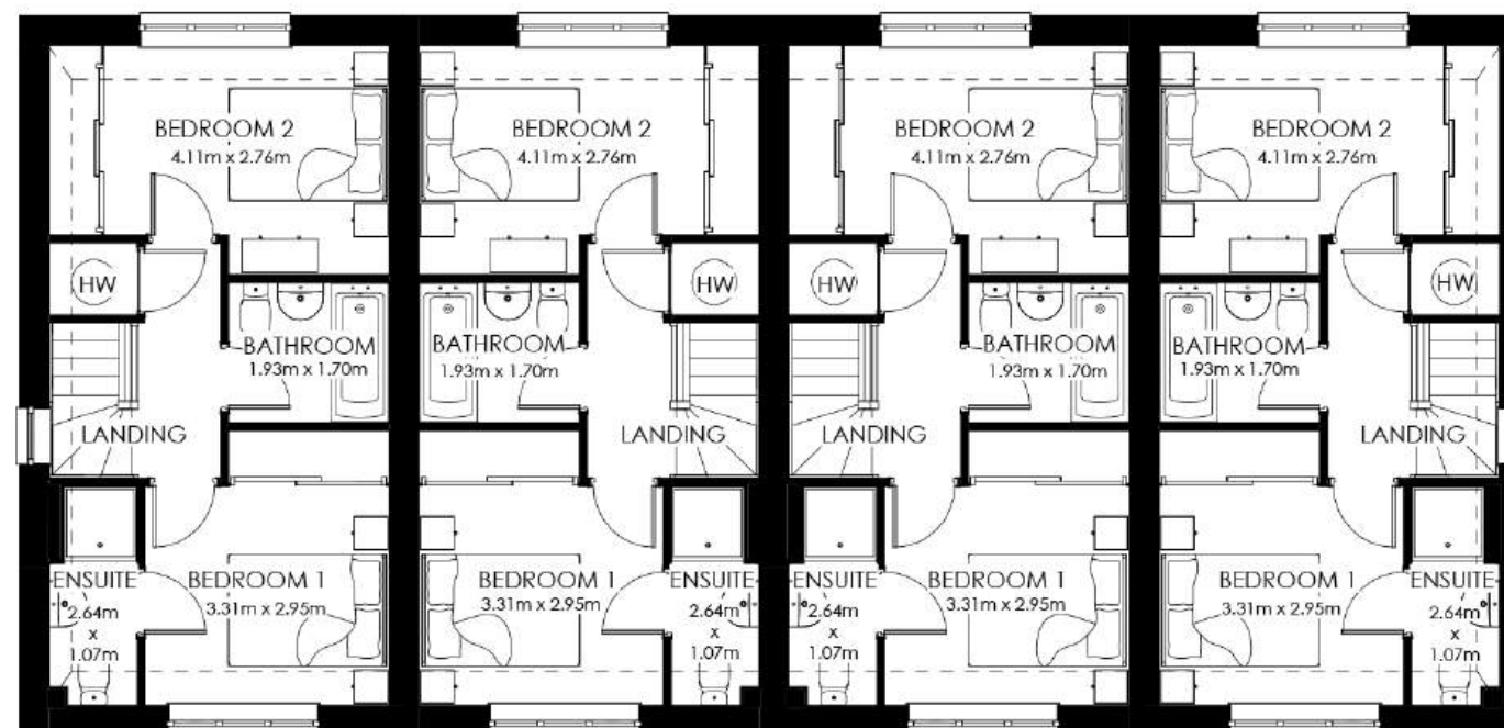
First Floor
