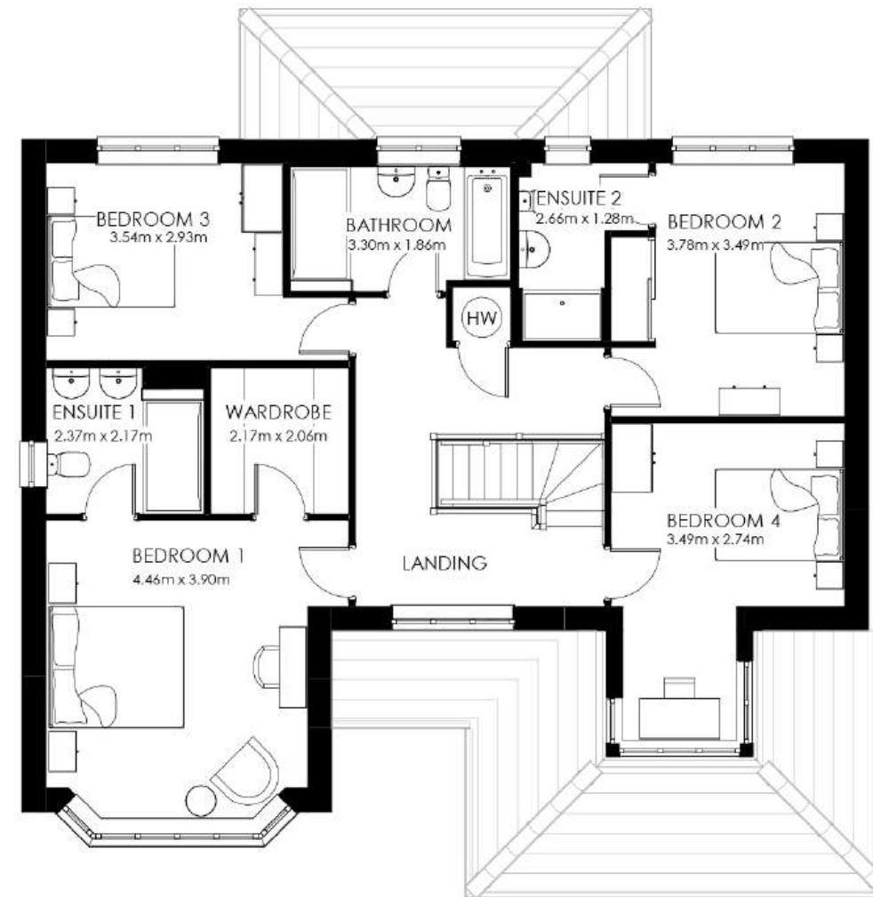
First Floor
