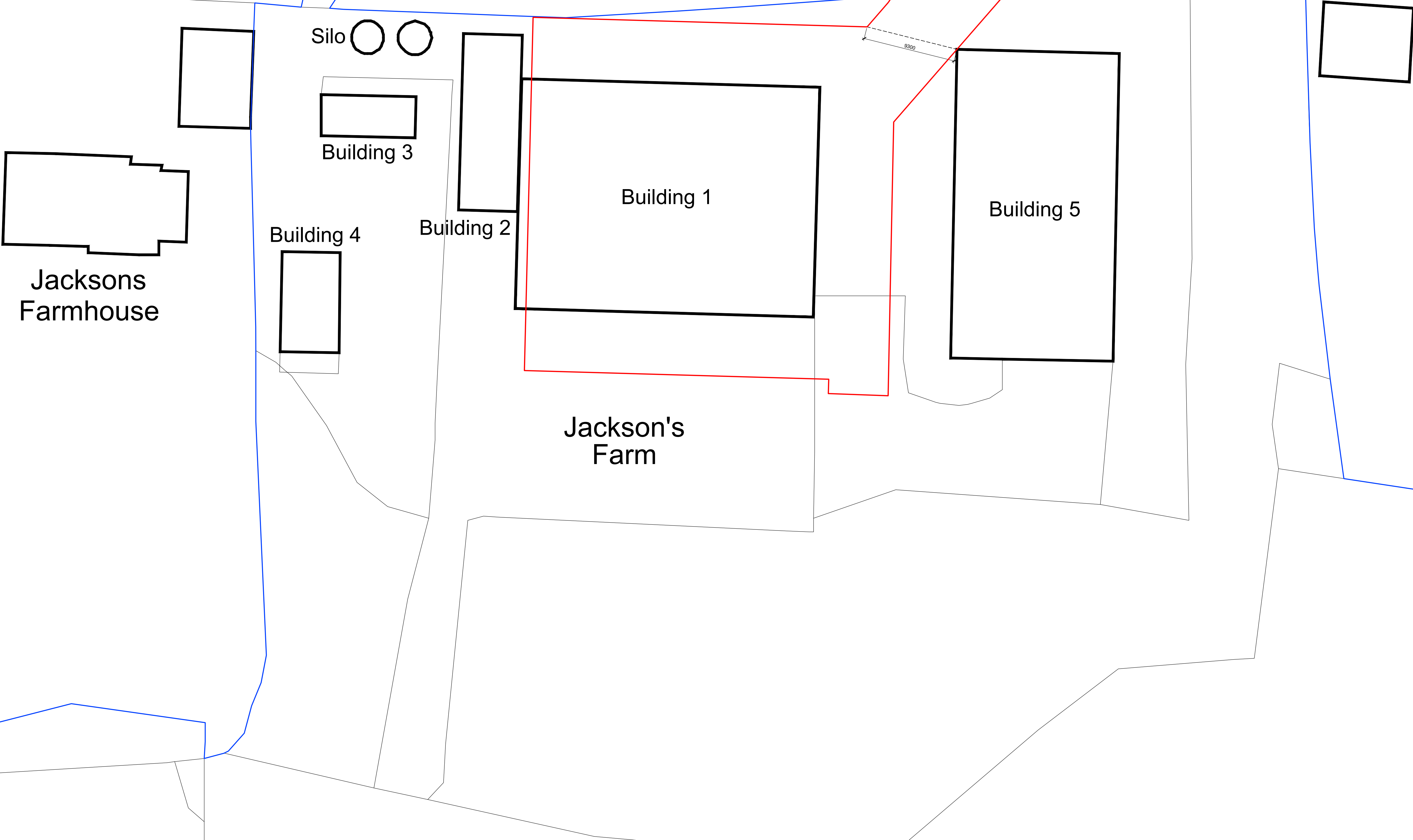
Existing Site Layout Plan (1:200)
