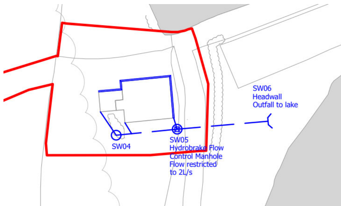
Figure 5.3: Area 6 Proposed Surface Water Drainage Strategy
