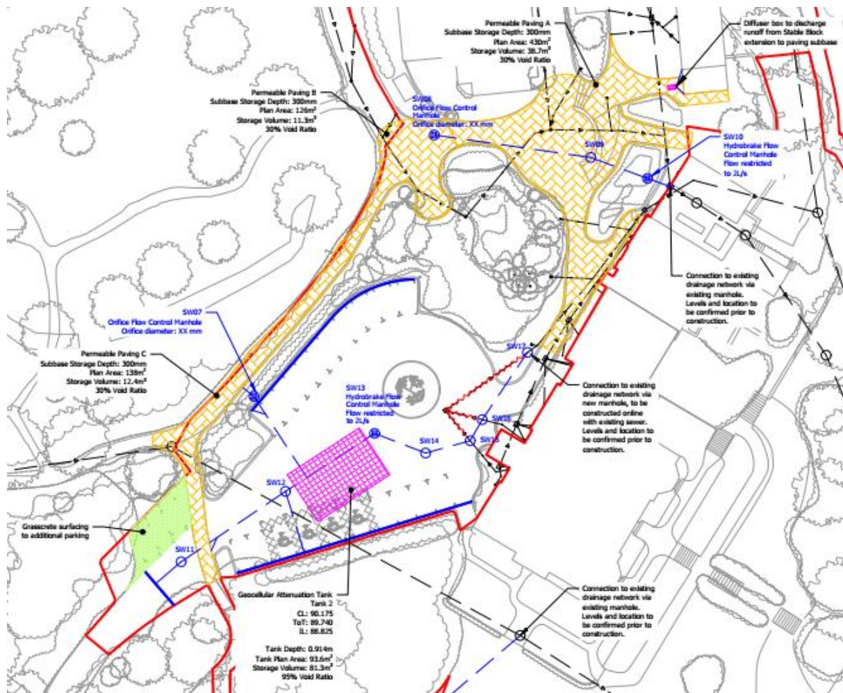
Figure 5.2: Area 2 Proposed Surface Water Drainage Strategy
