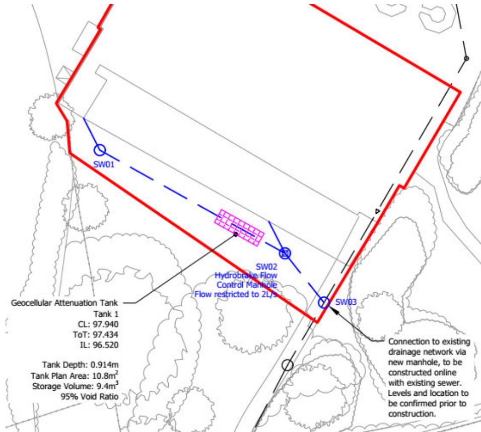
Figure 5.1: Area 1 Proposed Surface Water Drainage Strategy
