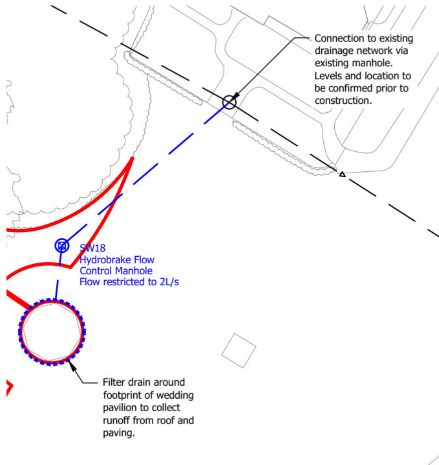
Figure 5.4: Area 6 Proposed Surface Water Drainage Strategy
