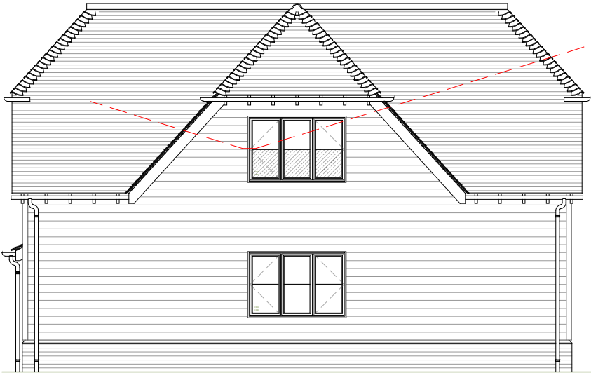
West 1:100 PROPOSED
