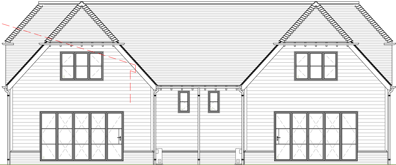
South 1:100 PROPOSED
