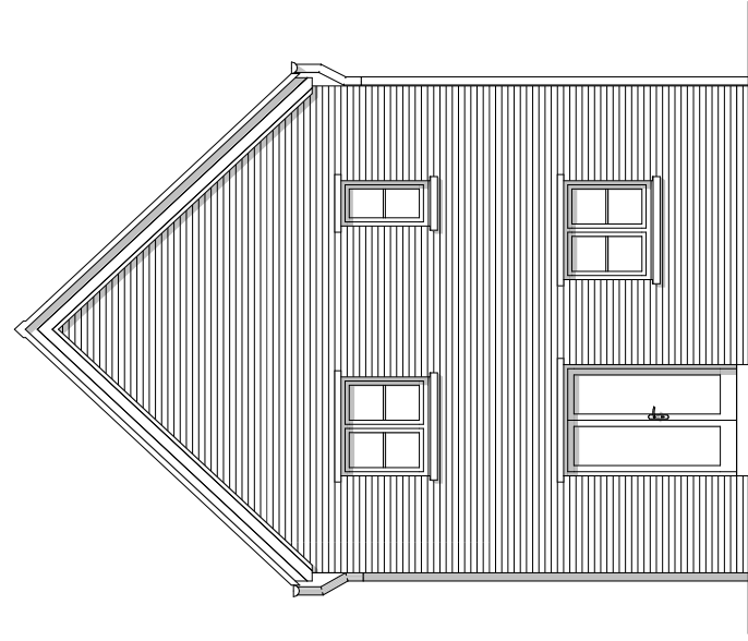
Rear Elevation
