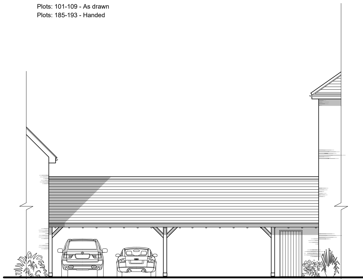
Rear Elevation
