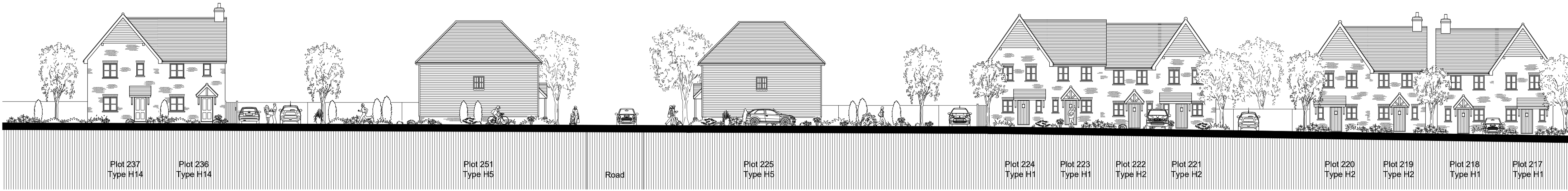
Section 19 - 19
