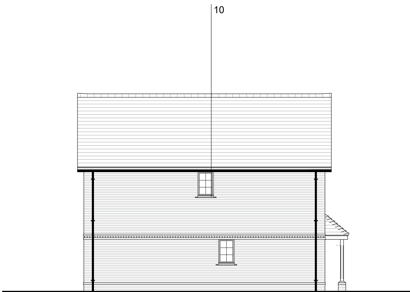
SIDE ELEVATION
