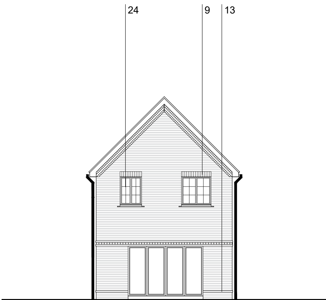
REAR ELEVATION
