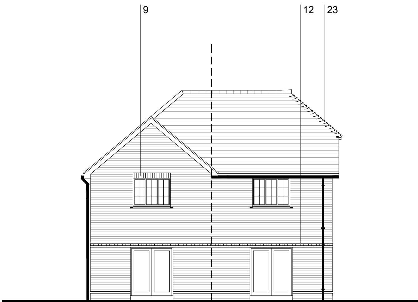
REAR ELEVATION
