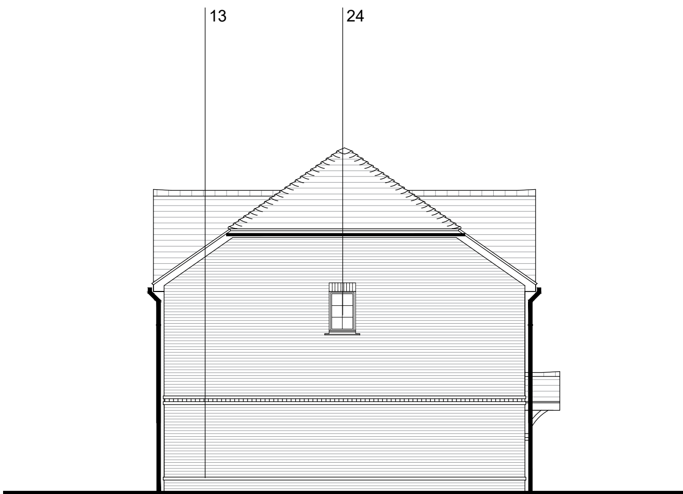
SIDE ELEVATION
