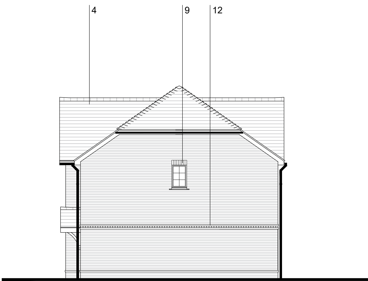
SIDE ELEVATION
