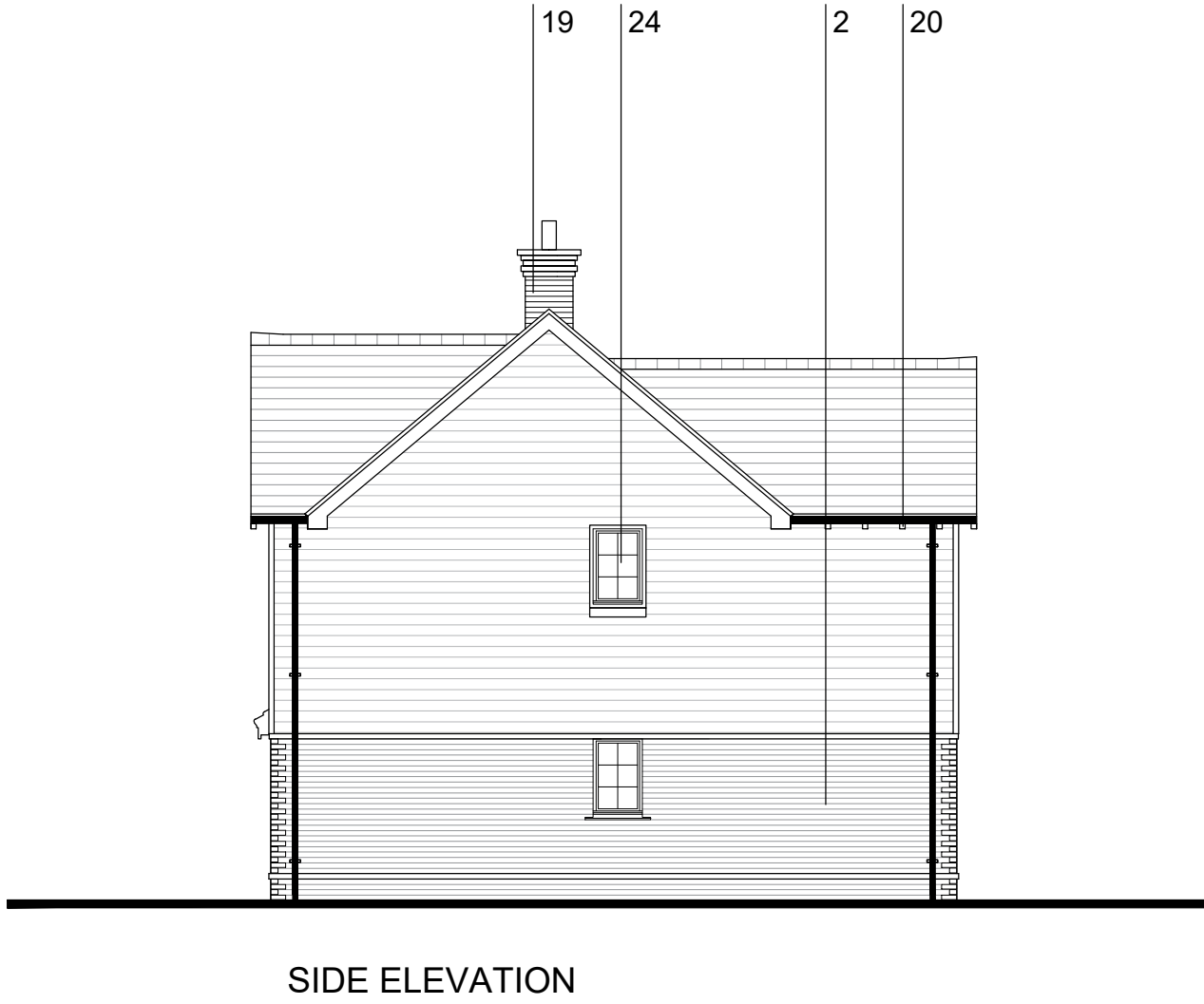
SIDE ELEVATION
