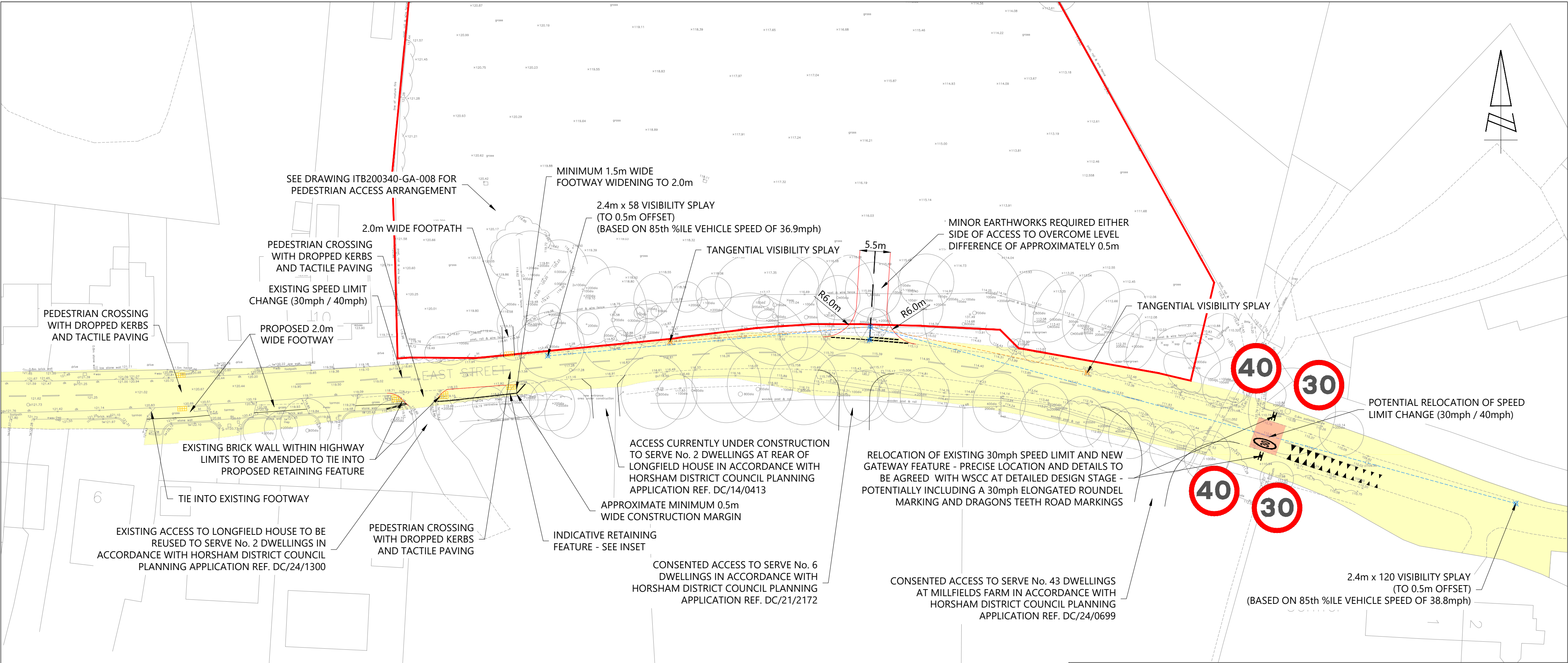
INSET - SCALE 1:25
