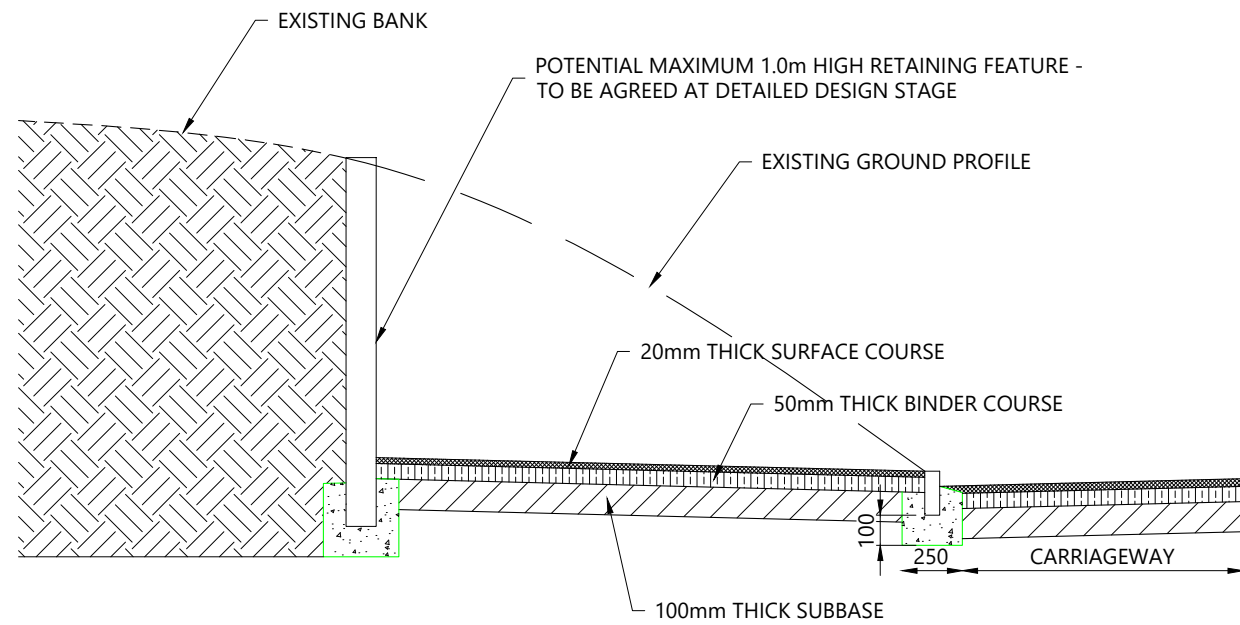
INDICATIVE FOOTWAY ROUTE STANDARD DETAIL
