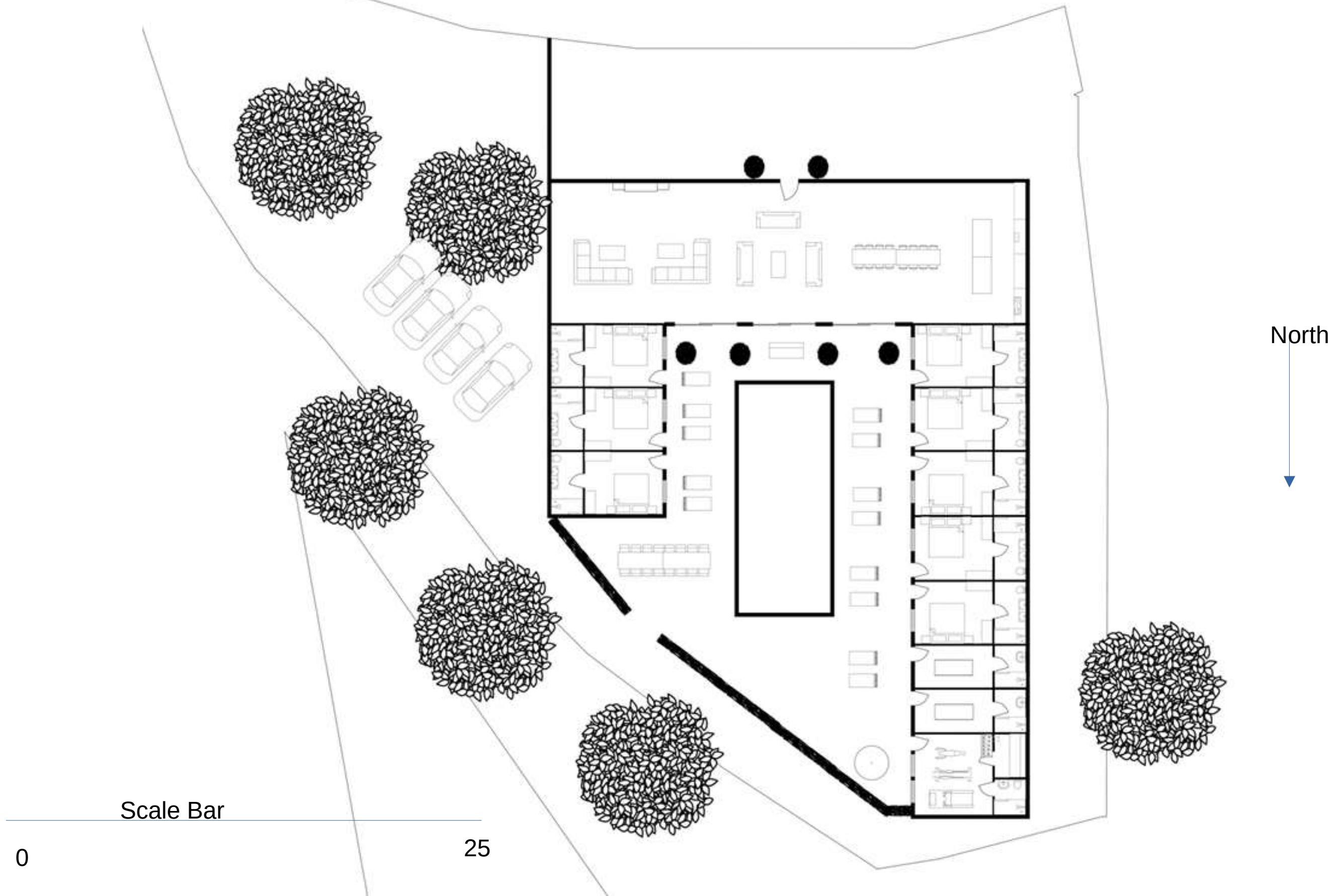
Proposed Floorplan – 1:200 at a3
