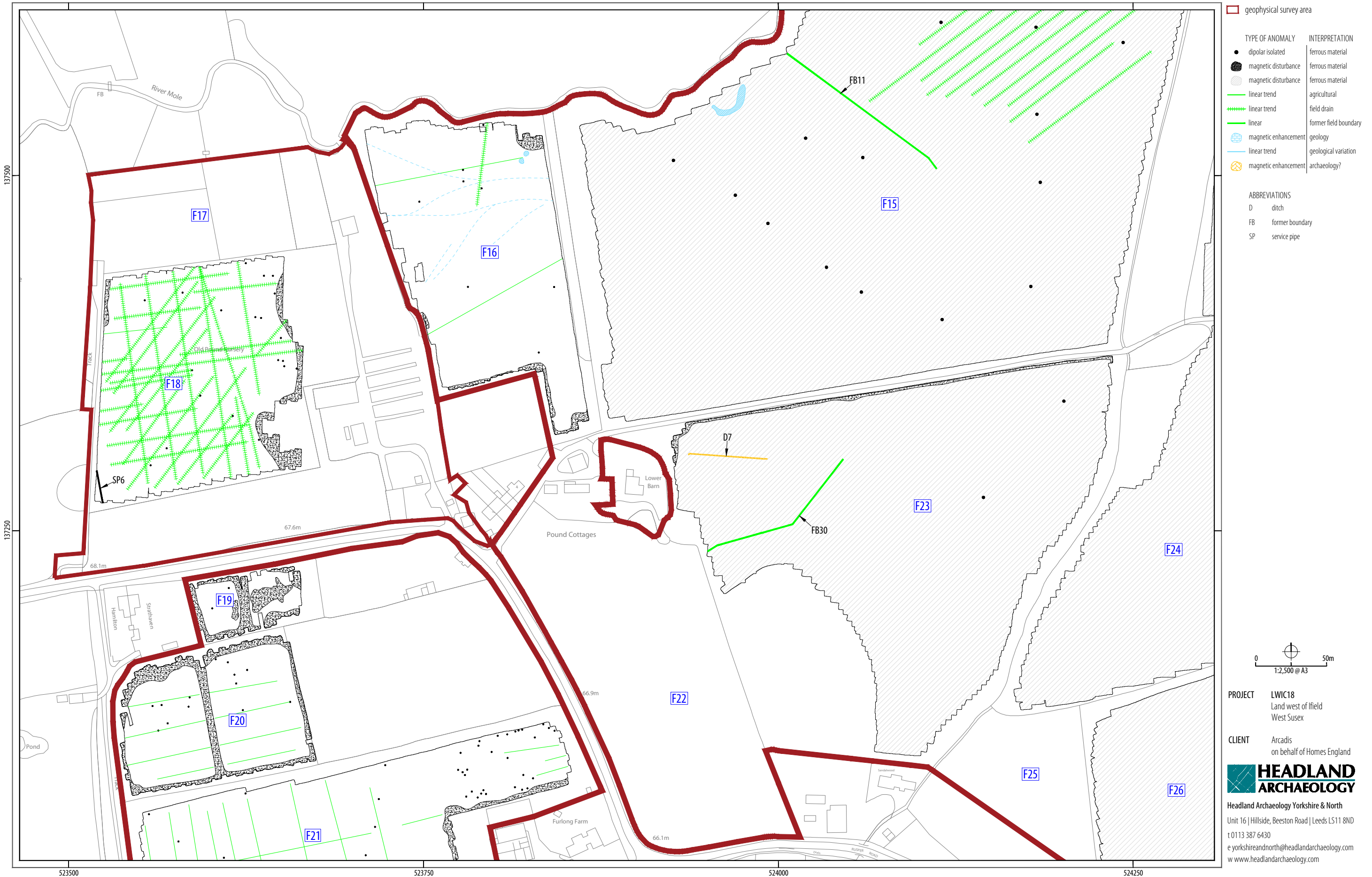
ILLUS 23 Interpretation of magnetometer data; Sector 4
