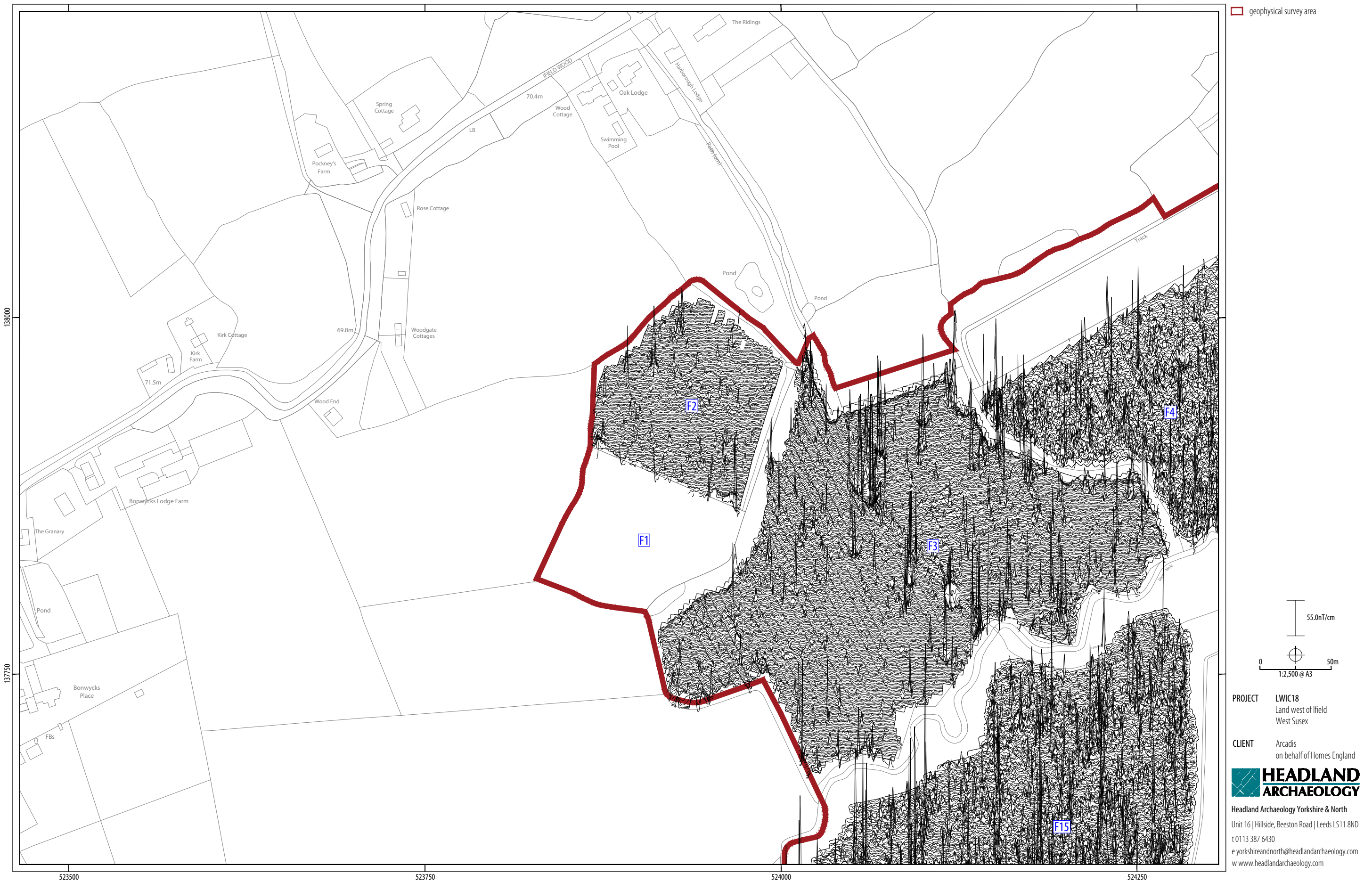
ILLUS 16 XY trace plot of minimally processed magnetometer data; Sector 2
