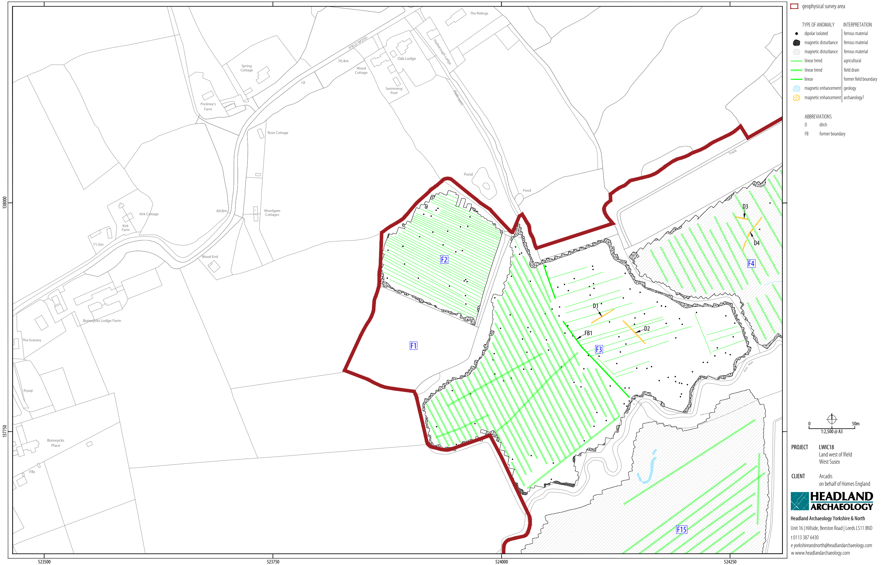
ILLUS 17 Interpretation of magnetometer data; Sector 2
