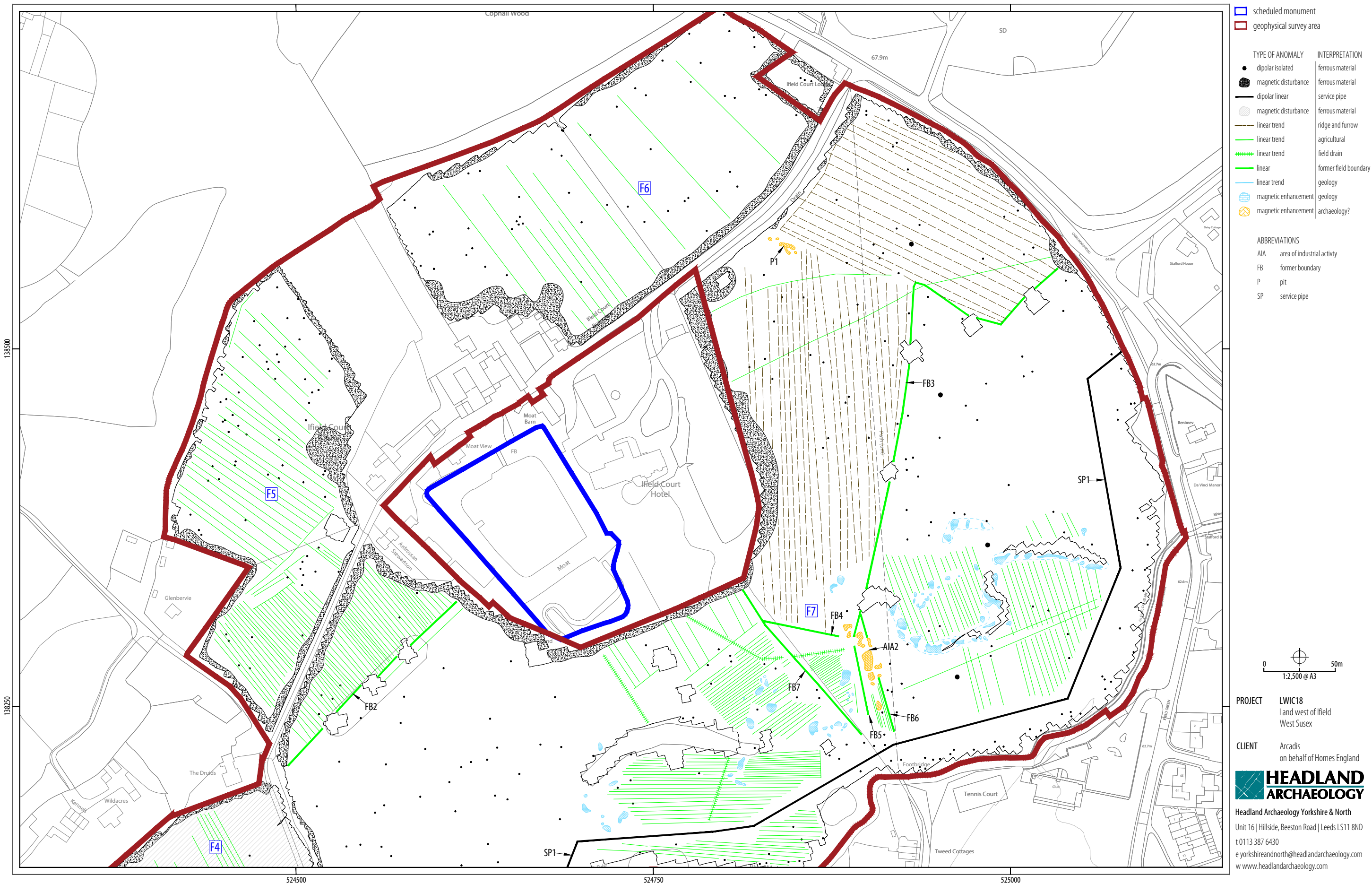
ILLUS 14 Interpretation of magnetometer data; Sector 1
