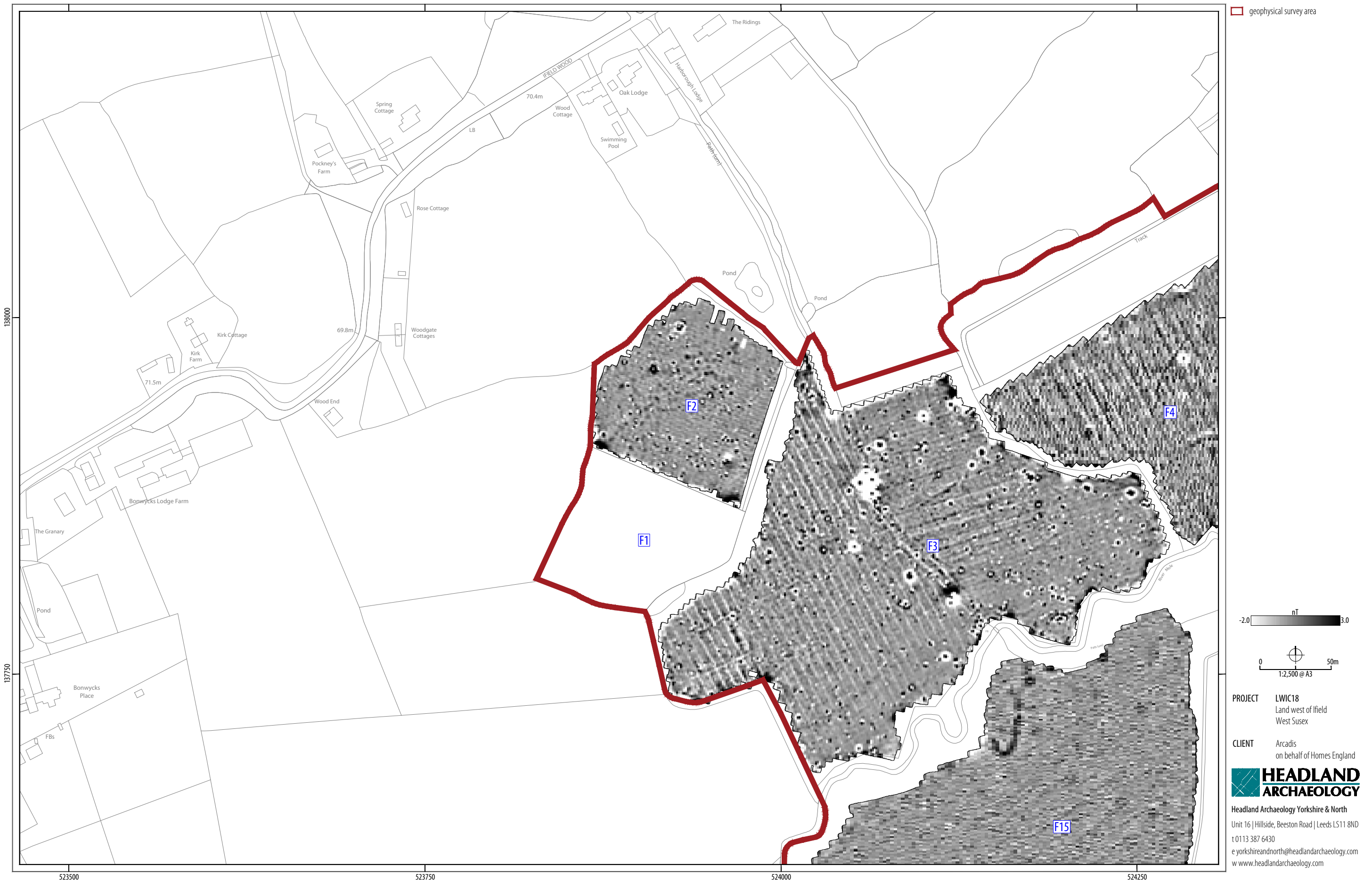
ILLUS 15 Processed greyscale magnetometer data; Sector 2
