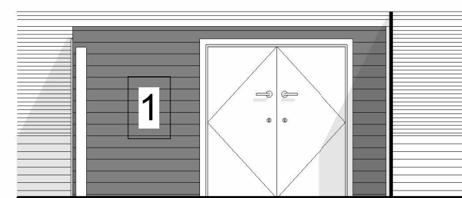
2.2 Type 2_Front View 1:50
