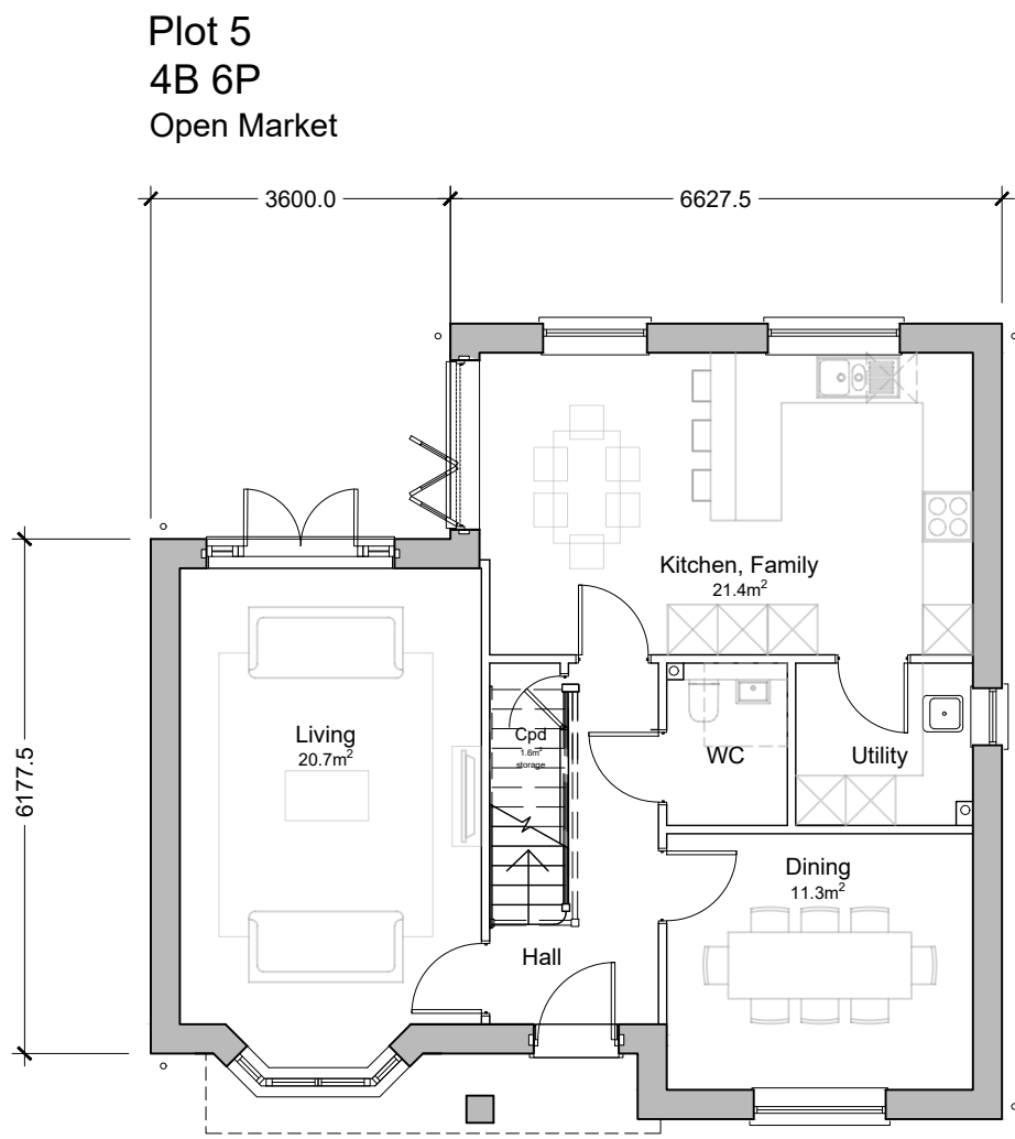
GROUND FLOOR
