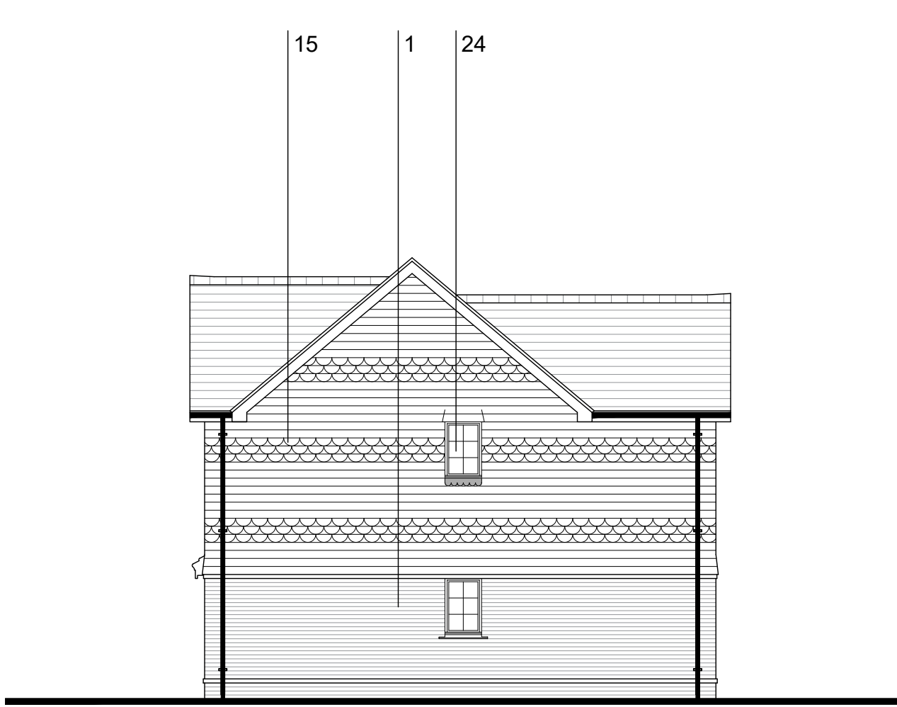
SIDE ELEVATION
