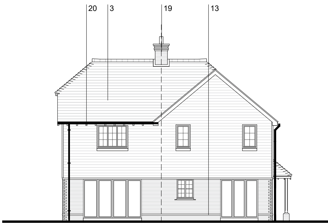
REAR ELEVATION
