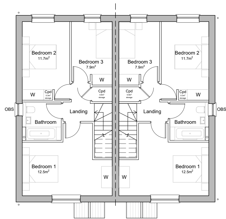
FIRST FLOOR
