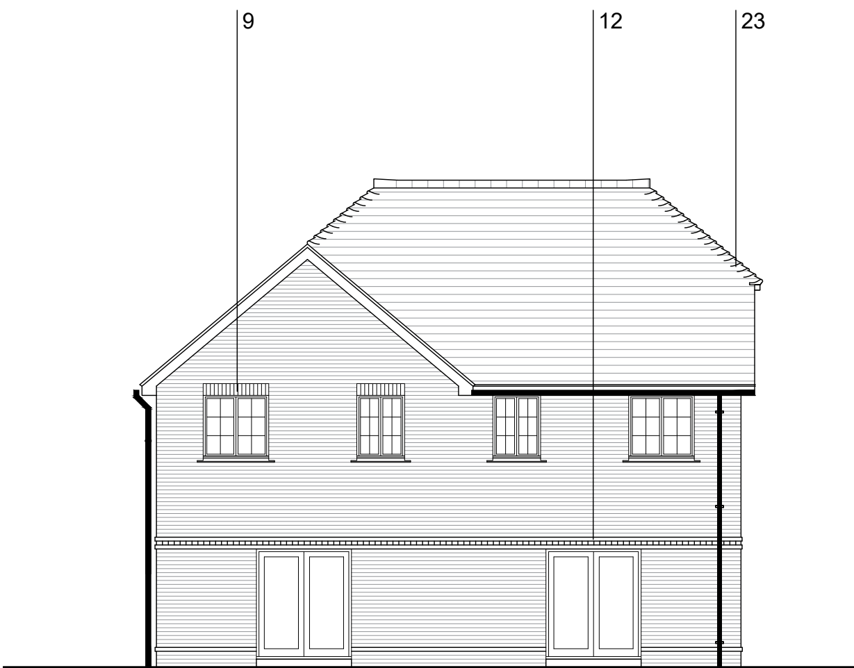
REAR ELEVATION
