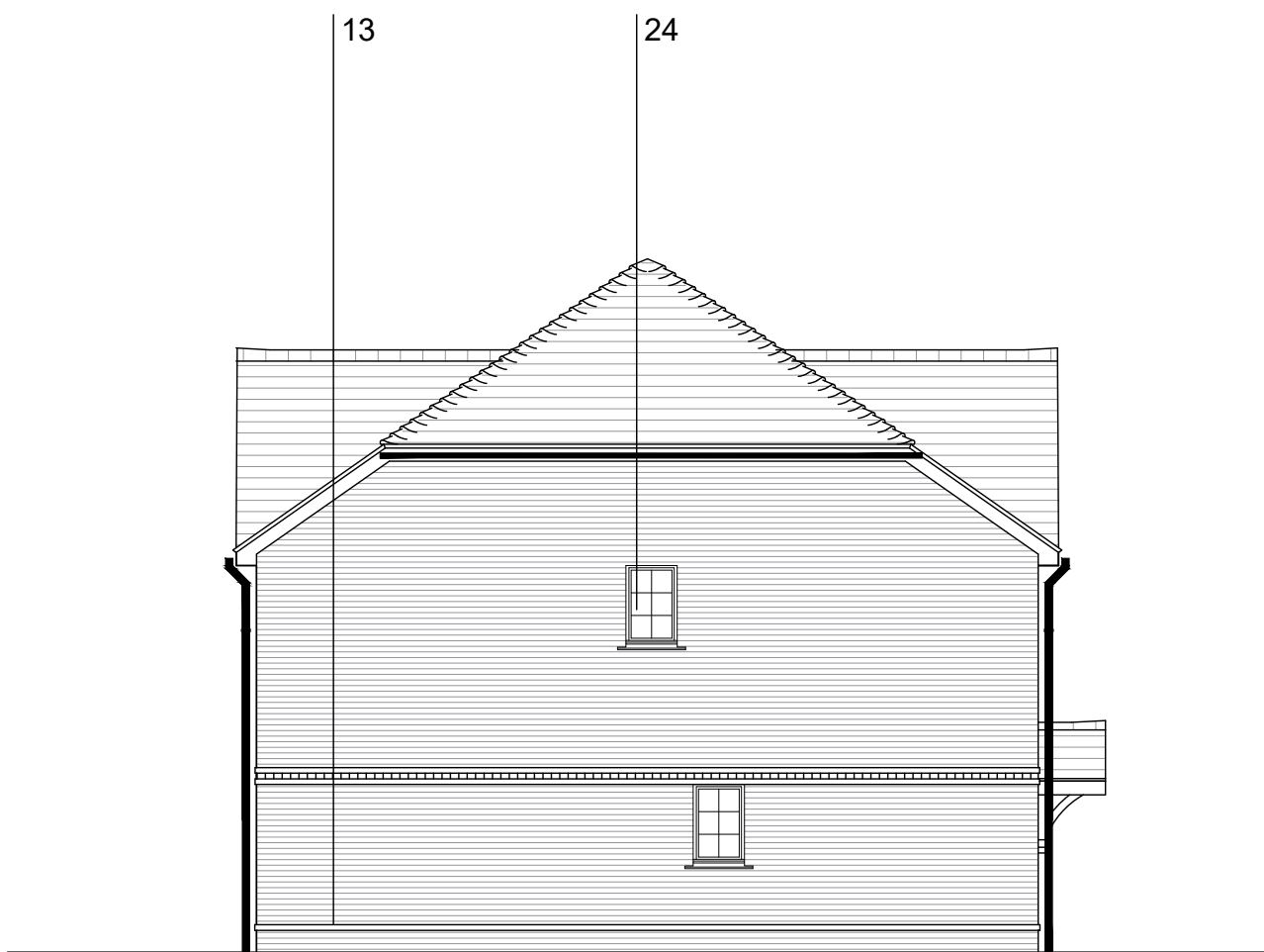
SIDE ELEVATION
