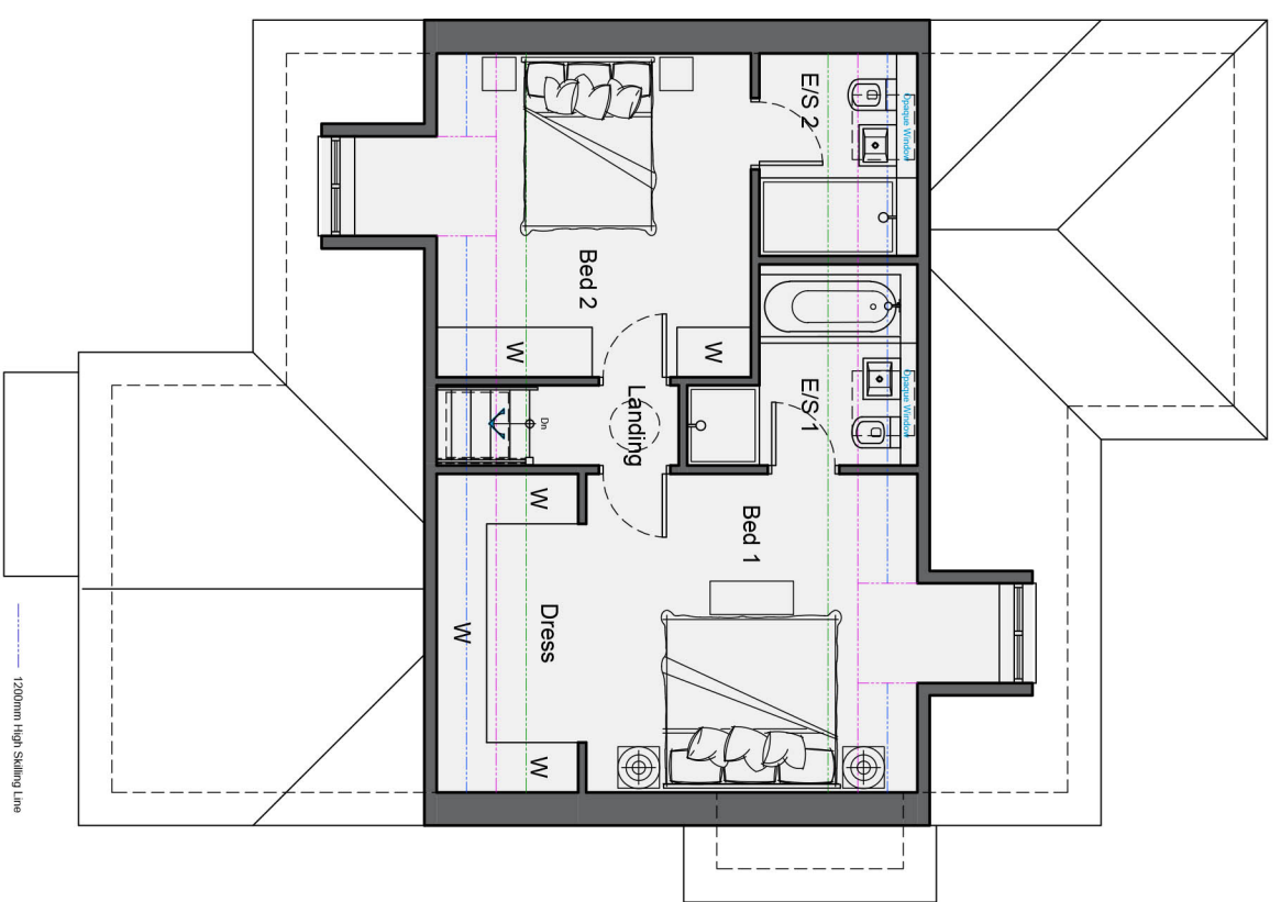
First Floor Plan GIA - 53.8m 2 (579ft 2 )
