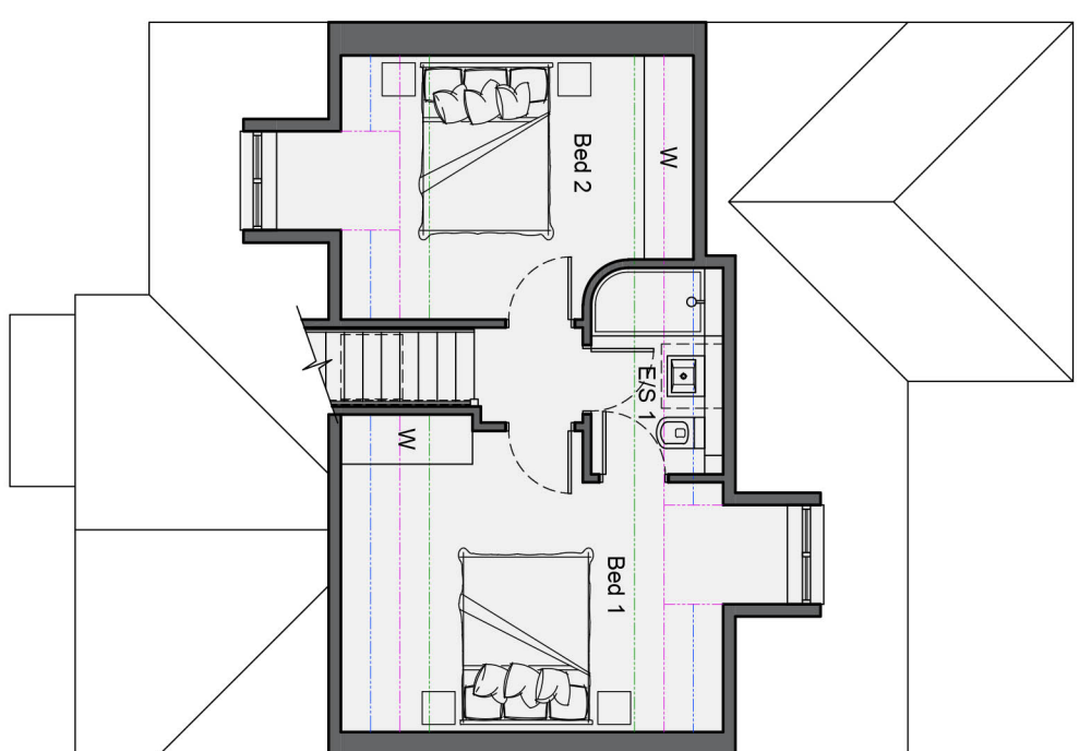
First Floor Plan GIA - 39.0m 2 (420ft 2 )
