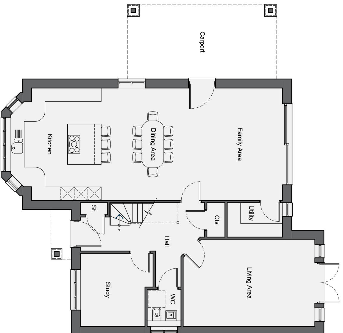
Ground Floor Plan GIA - 114.8m 2 (1,236ft 2 ) TOTAL GIA - 212.7m 2 (2,290ft 2 )
